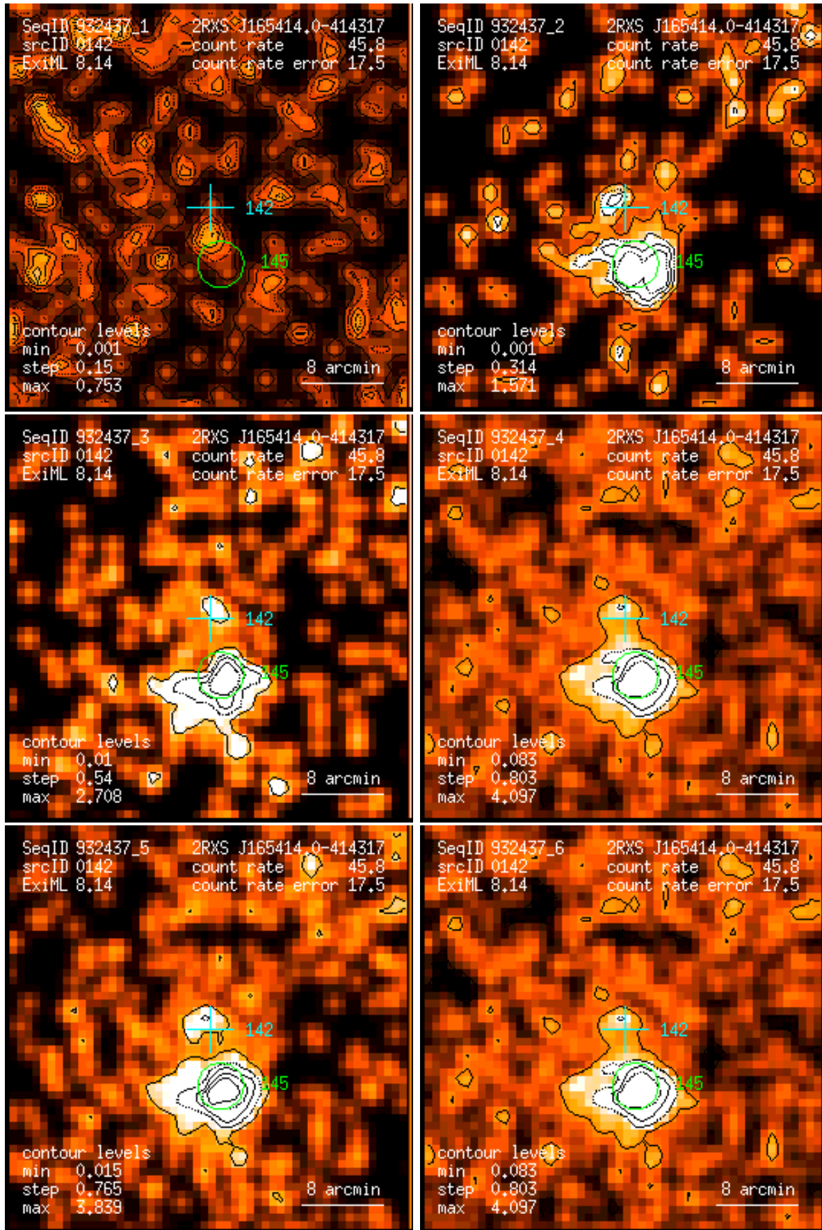
Figure 142: RASS 932437: detection 0142: band rate images, Gaussian filter: (1) PSPC channels 11 – 41, (2) 52 – 90, (3) 91 – 201, (4) 11 – 235, (5) 52 – 201, (6) 11 – 201. Broad band rates in counts/ks. Band rate contour levels in counts/ks/arcmin 2 .
