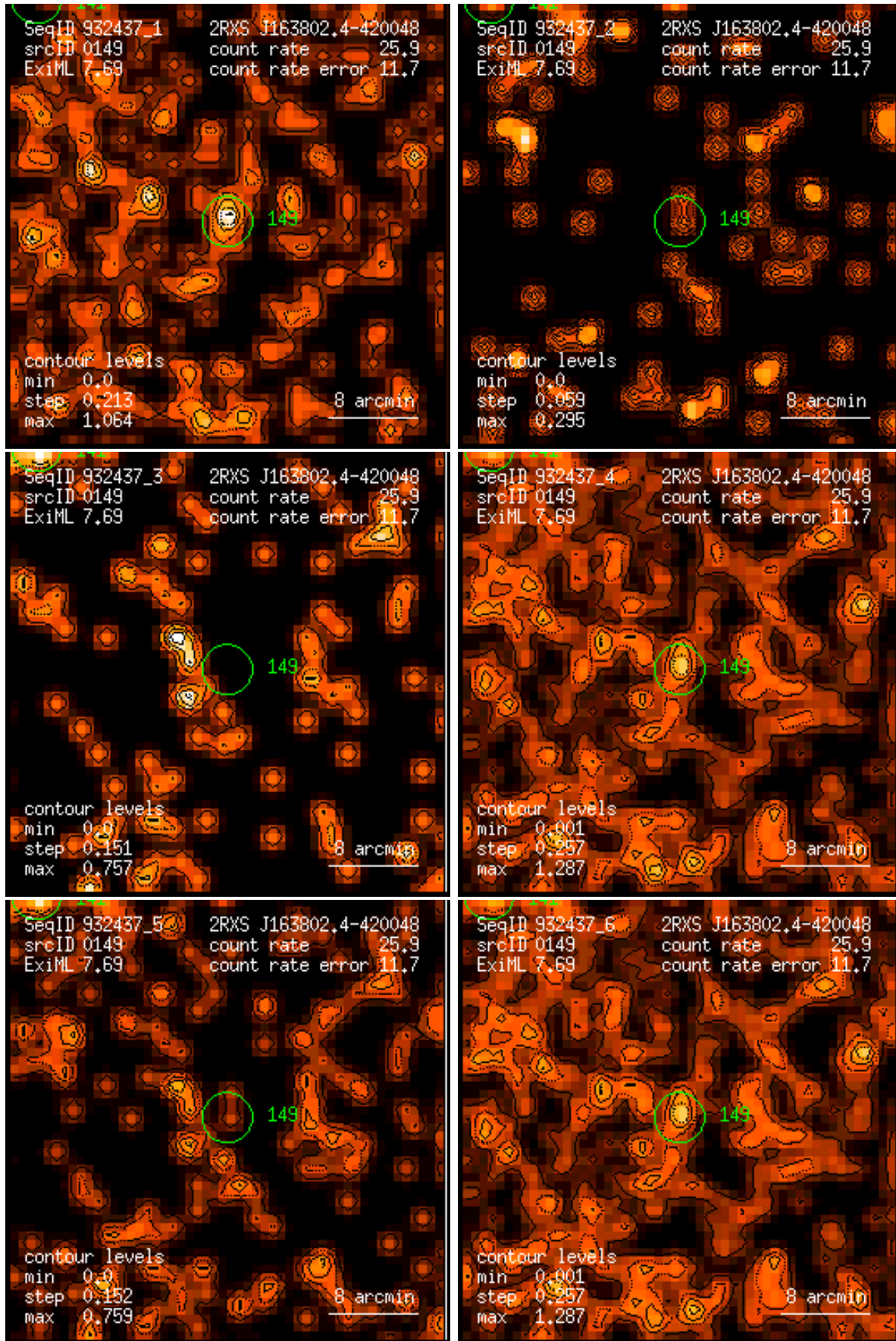
Figure 149: RASS 932437: detection 0149: band rate images, Gaussian filter: (1) PSPC channels 11 – 41, (2) 52 – 90, (3) 91 – 201, (4) 11 – 235, (5) 52 – 201, (6) 11 – 201. Broad band rates in counts/ks. Band rate contour levels in counts/ks/arcmin 2 .
