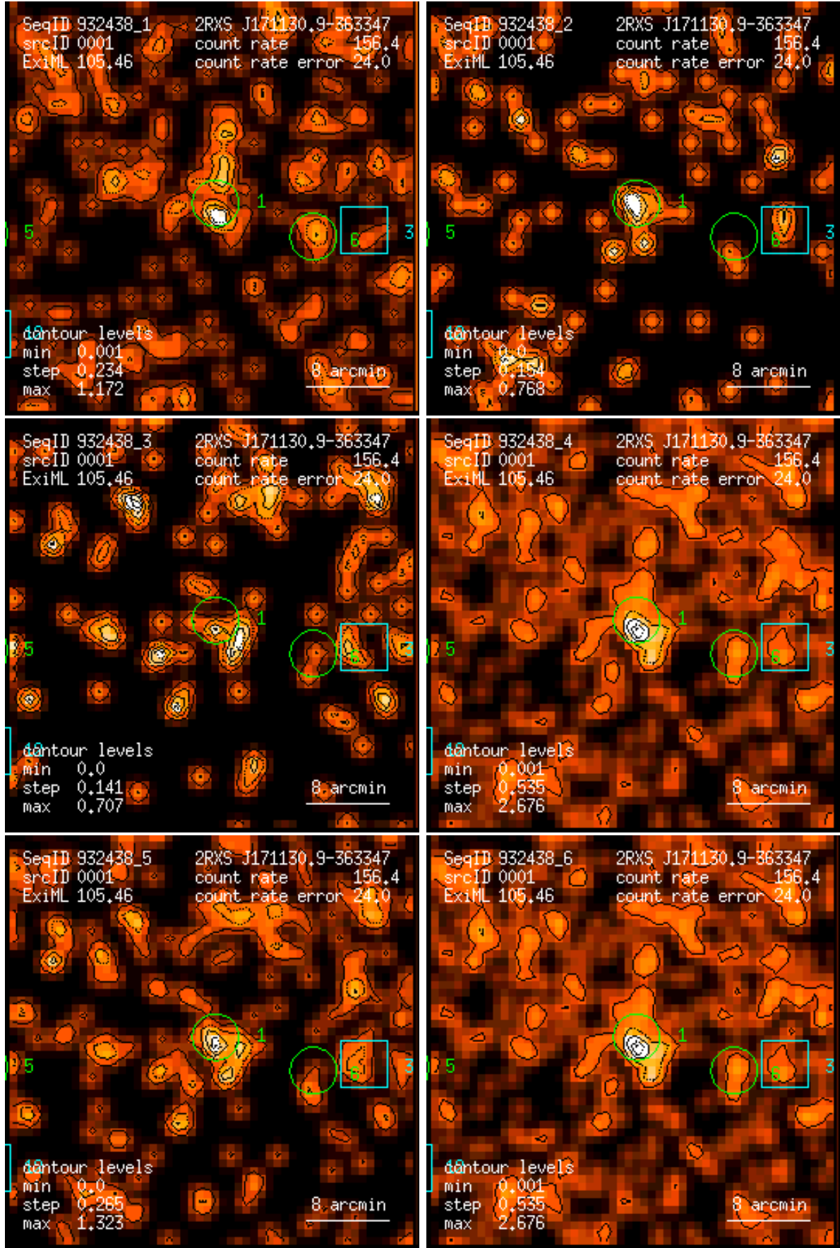
Figure 1: RASS 932438: detection 0001: band rate images, Gaussian filter: (1) PSPC channels 11 – 41, (2) 52 – 90, (3) 91 – 201, (4) 11 – 235, (5) 52 – 201, (6) 11 – 201. Broad band rates in counts/ks. Band rate contour levels in counts/ks/arcmin 2 .
