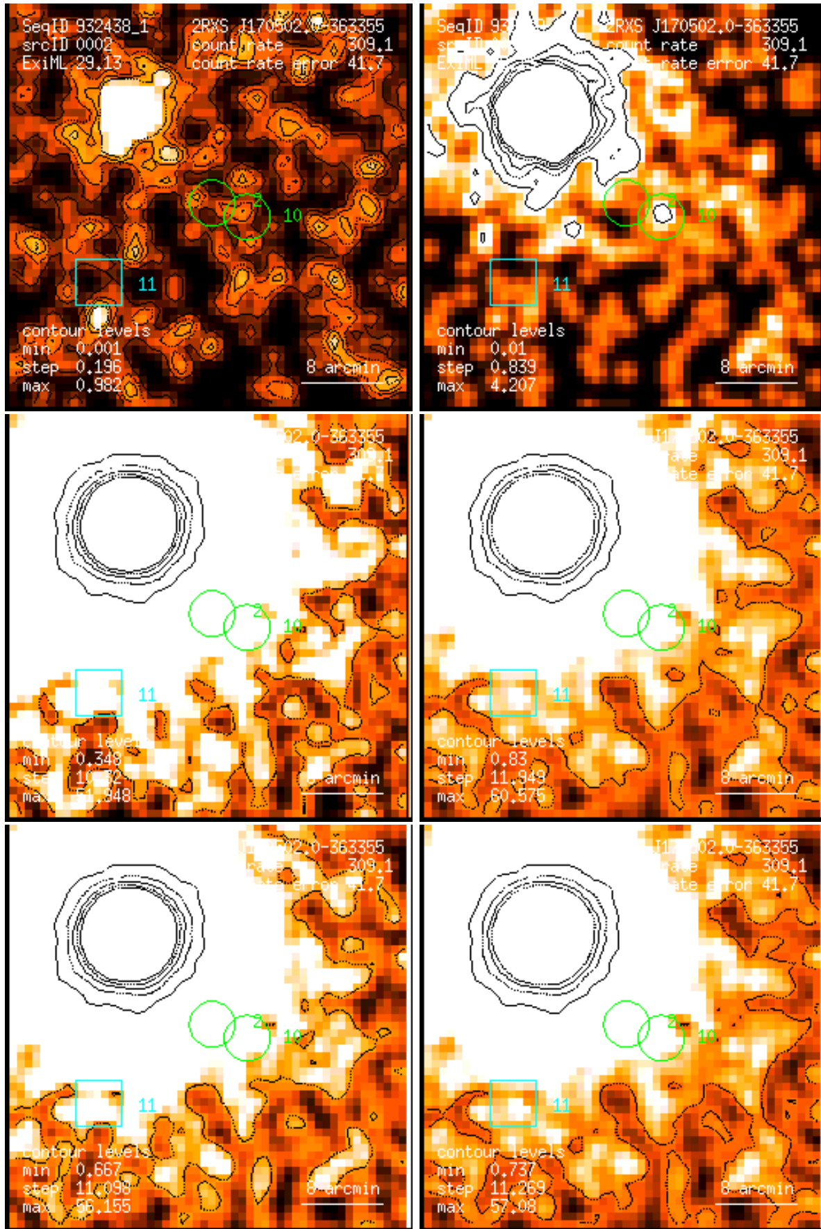
Figure 2: RASS 932438: detection 0002: band rate images, Gaussian filter: (1) PSPC channels 11 – 41, (2) 52 – 90, (3) 91 – 201, (4) 11 – 235, (5) 52 – 201, (6) 11 – 201. Broad band rates in counts/ks. Band rate contour levels in counts/ks/arcmin 2 .
