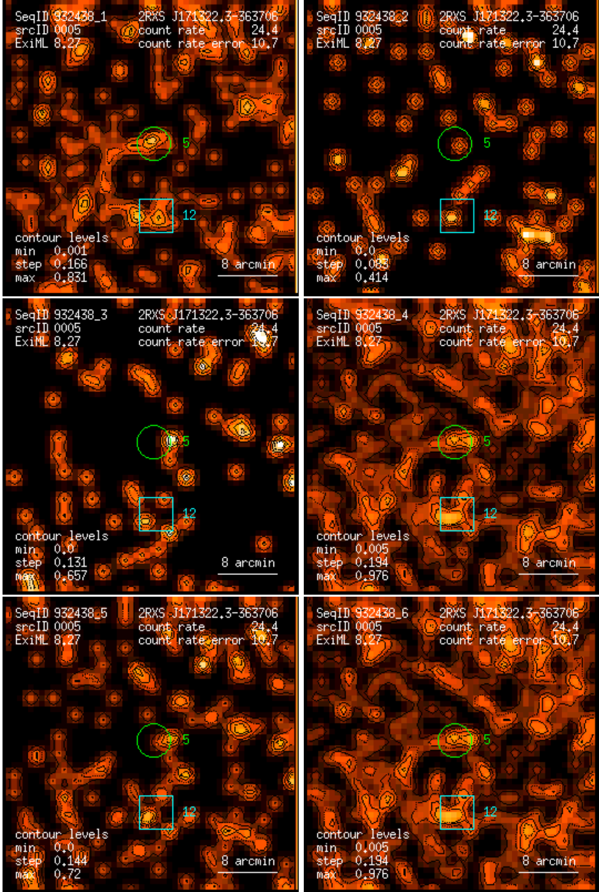
Figure 5: RASS 932438: detection 0005: band rate images, Gaussian filter: (1) PSPC channels 11 – 41, (2) 52 – 90, (3) 91 – 201, (4) 11 – 235, (5) 52 – 201, (6) 11 – 201. Broad band rates in counts/ks. Band rate contour levels in counts/ks/arcmin 2 .
