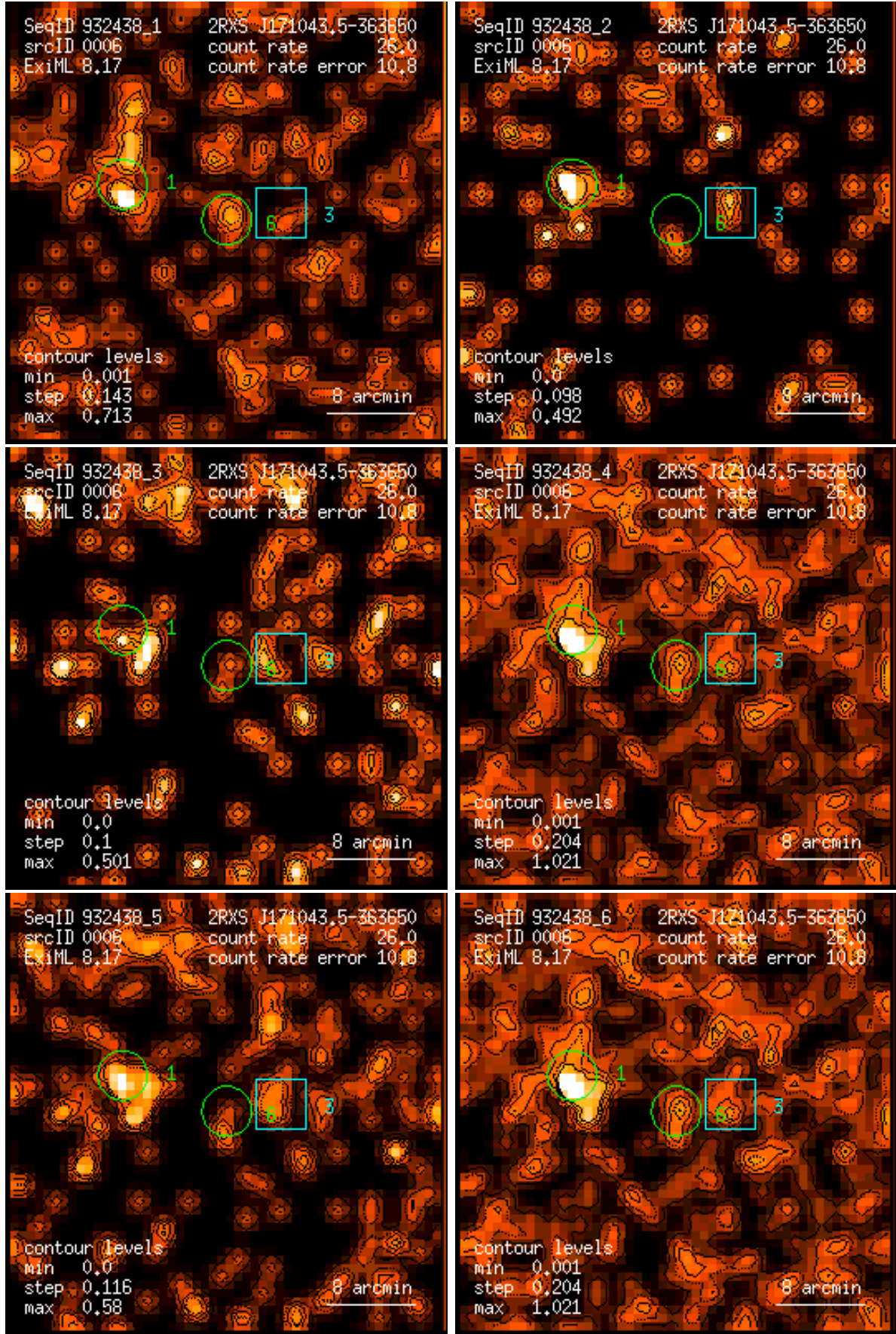
Figure 6: RASS 932438: detection 0006: band rate images, Gaussian filter: (1) PSPC channels 11 – 41, (2) 52 – 90, (3) 91 – 201, (4) 11 – 235, (5) 52 – 201, (6) 11 – 201. Broad band rates in counts/ks. Band rate contour levels in counts/ks/arcmin 2 .
