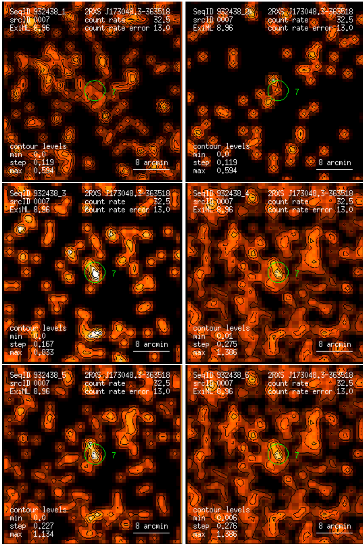
Figure 7: RASS 932438: detection 0007: band rate images, Gaussian filter: (1) PSPC channels 11 – 41, (2) 52 – 90, (3) 91 – 201, (4) 11 – 235, (5) 52 – 201, (6) 11 – 201. Broad band rates in counts/ks. Band rate contour levels in counts/ks/arcmin 2 .
