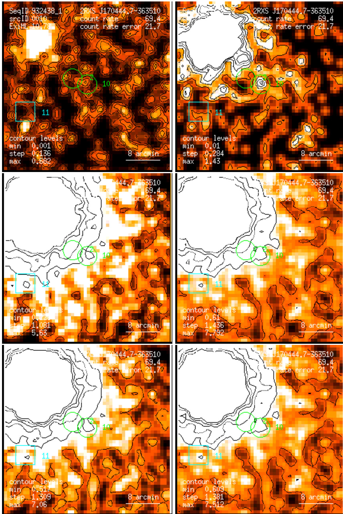
Figure 10: RASS 932438: detection 0010: band rate images, Gaussian filter: (1) PSPC channels 11 – 41, (2) 52 – 90, (3) 91 – 201, (4) 11 – 235, (5) 52 – 201, (6) 11 – 201. Broad band rates in counts/ks. Band rate contour levels in counts/ks/arcmin 2 .
