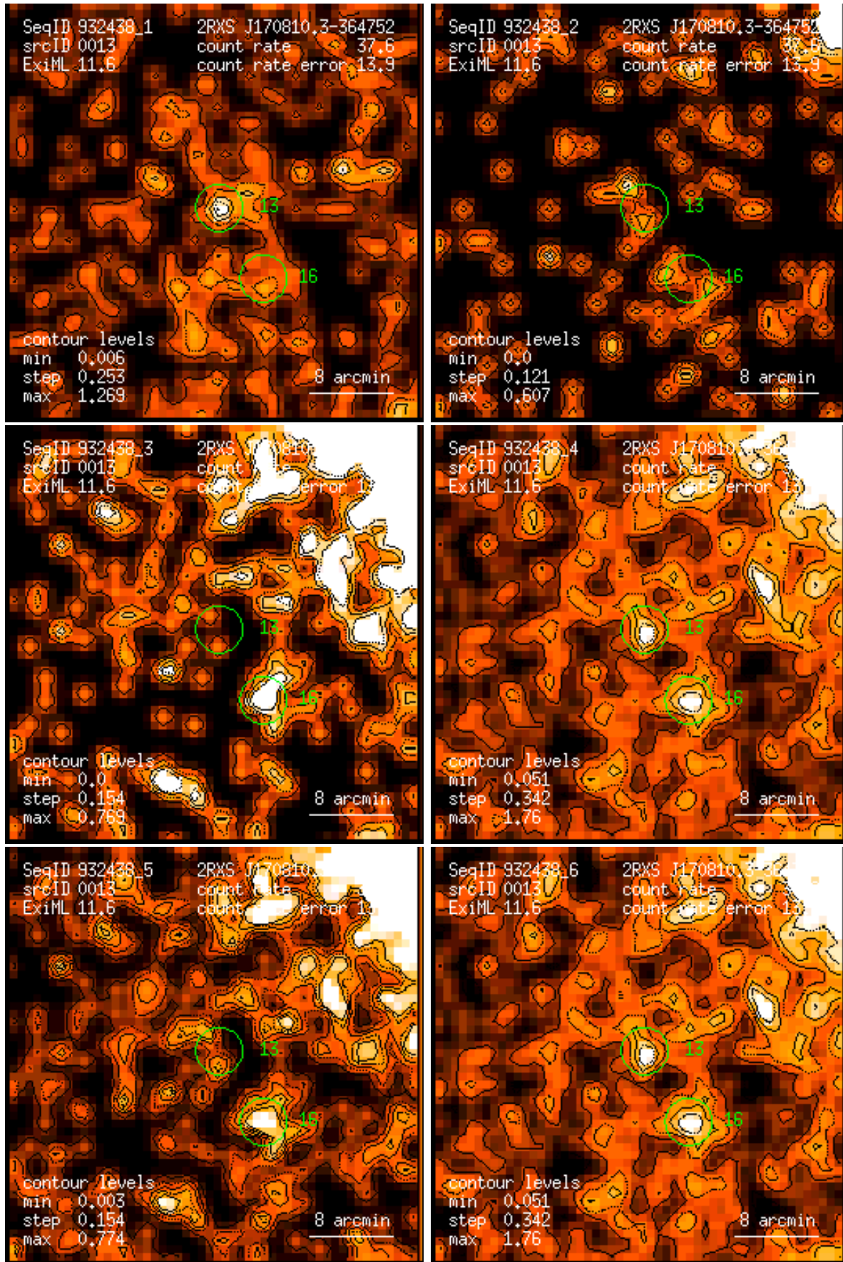
Figure 13: RASS 932438: detection 0013: band rate images, Gaussian filter: (1) PSPC channels 11 – 41, (2) 52 – 90, (3) 91 – 201, (4) 11 – 235, (5) 52 – 201, (6) 11 – 201. Broad band rates in counts/ks. Band rate contour levels in counts/ks/arcmin 2 .
