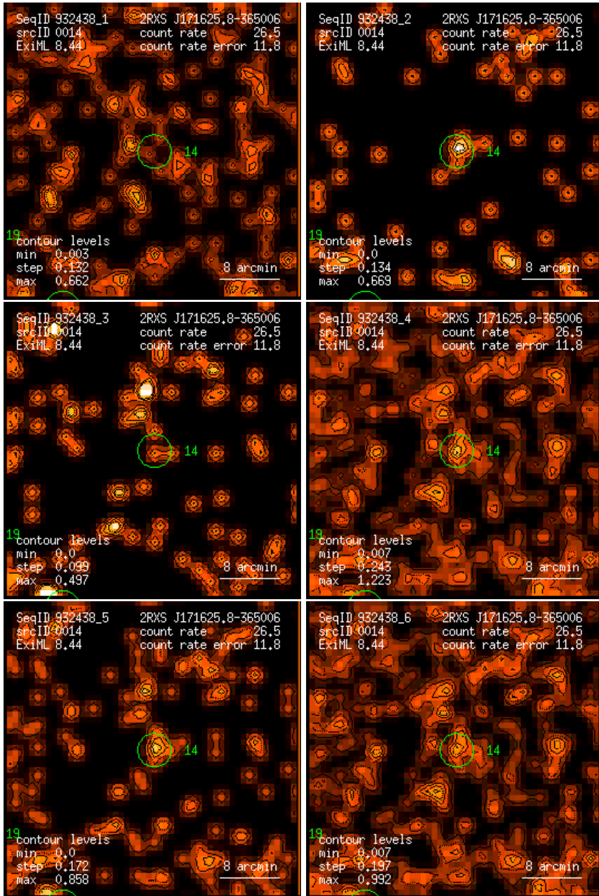
Figure 14: RASS 932438: detection 0014: band rate images, Gaussian filter: (1) PSPC channels 11 – 41, (2) 52 – 90, (3) 91 – 201, (4) 11 – 235, (5) 52 – 201, (6) 11 – 201. Broad band rates in counts/ks. Band rate contour levels in counts/ks/arcmin 2 .
