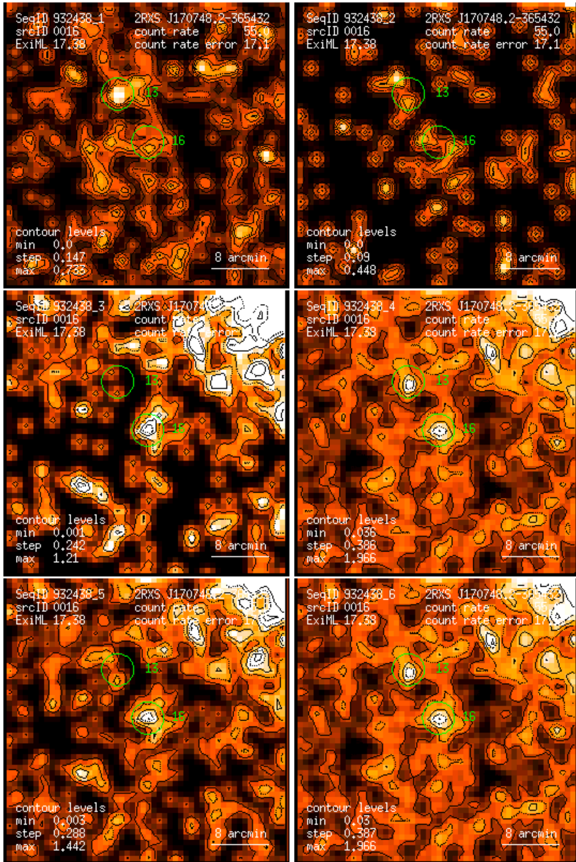
Figure 16: RASS 932438: detection 0016: band rate images, Gaussian filter: (1) PSPC channels 11 – 41, (2) 52 – 90, (3) 91 – 201, (4) 11 – 235, (5) 52 – 201, (6) 11 – 201. Broad band rates in counts/ks. Band rate contour levels in counts/ks/arcmin 2 .
