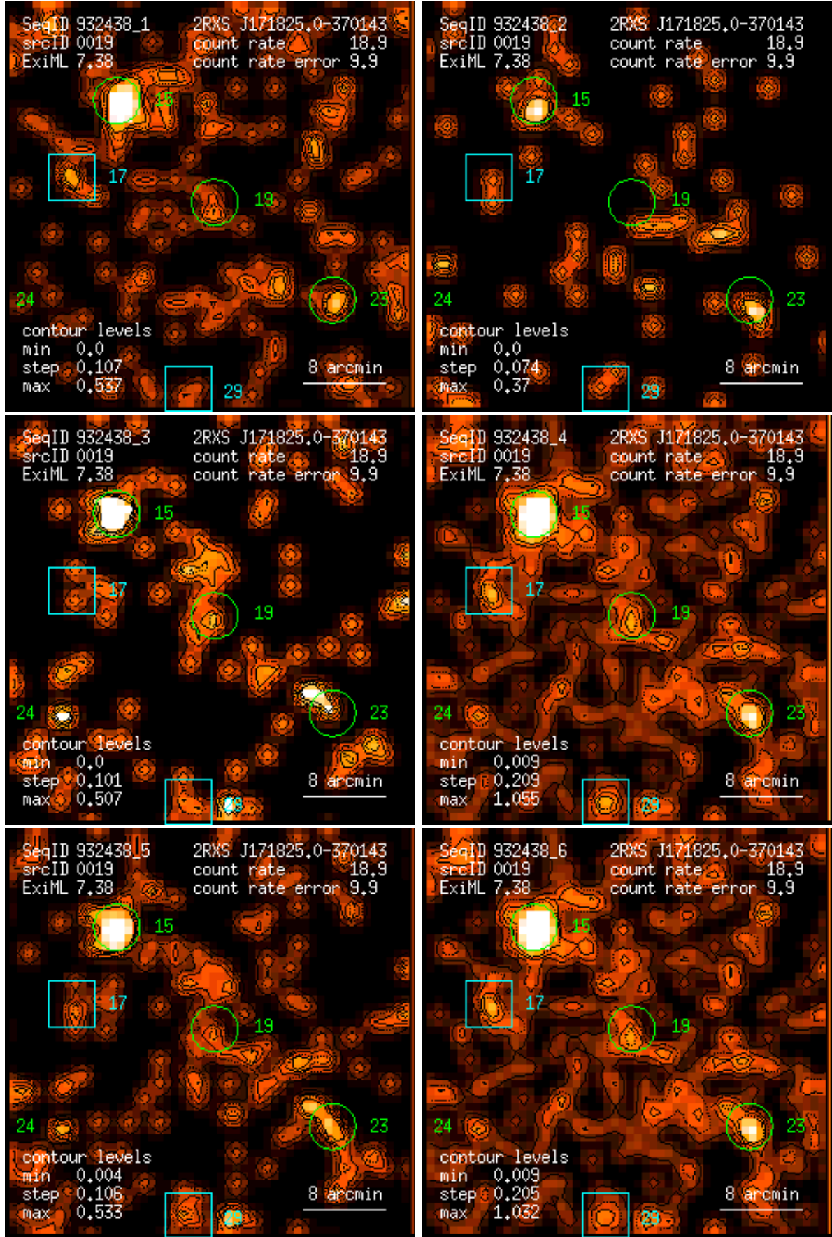
Figure 19: RASS 932438: detection 0019: band rate images, Gaussian filter: (1) PSPC channels 11 – 41, (2) 52 – 90, (3) 91 – 201, (4) 11 – 235, (5) 52 – 201, (6) 11 – 201. Broad band rates in counts/ks. Band rate contour levels in counts/ks/arcmin 2 .
