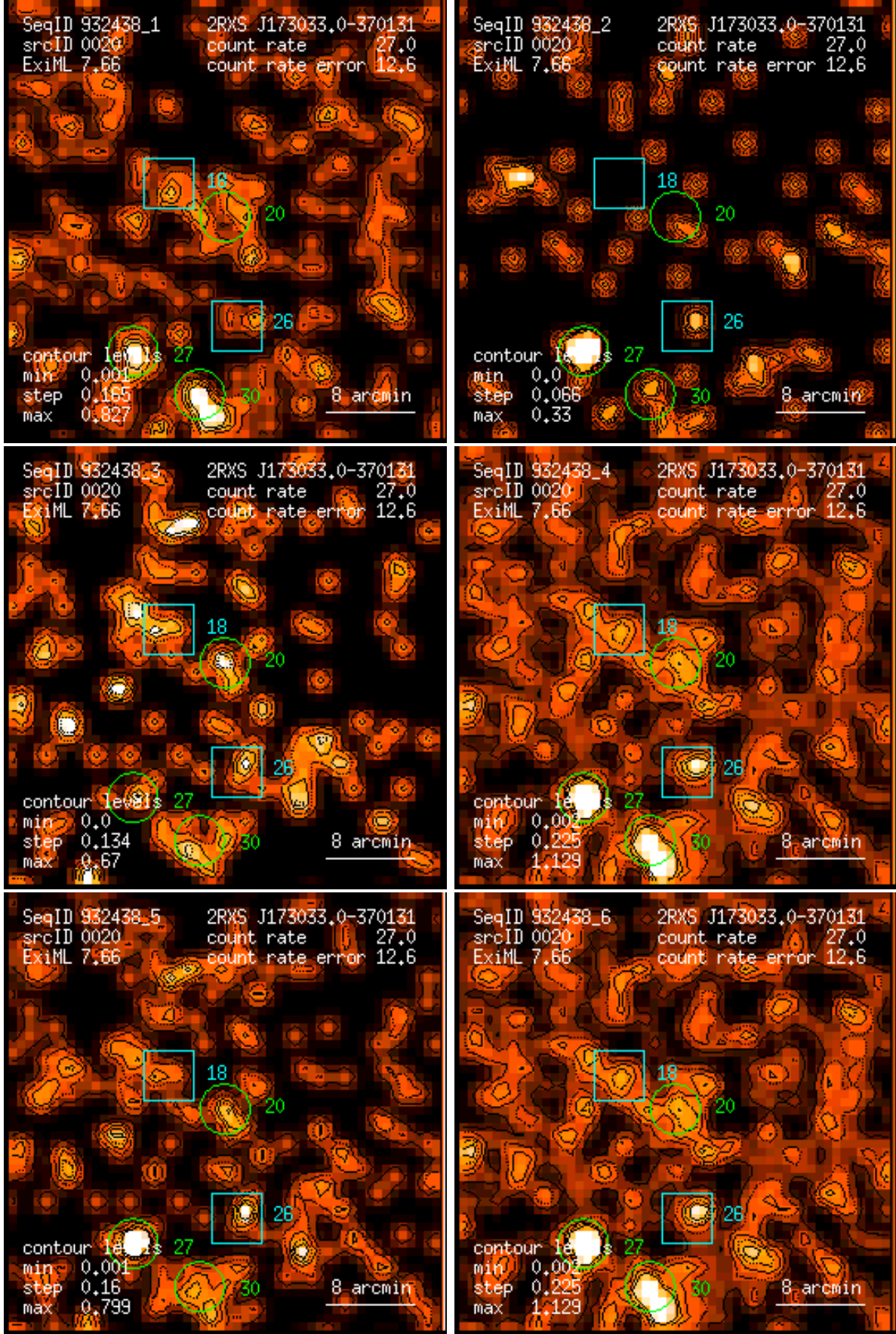
Figure 20: RASS 932438: detection 0020: band rate images, Gaussian filter: (1) PSPC channels 11 – 41, (2) 52 – 90, (3) 91 – 201, (4) 11 – 235, (5) 52 – 201, (6) 11 – 201. Broad band rates in counts/ks. Band rate contour levels in counts/ks/arcmin 2 .
