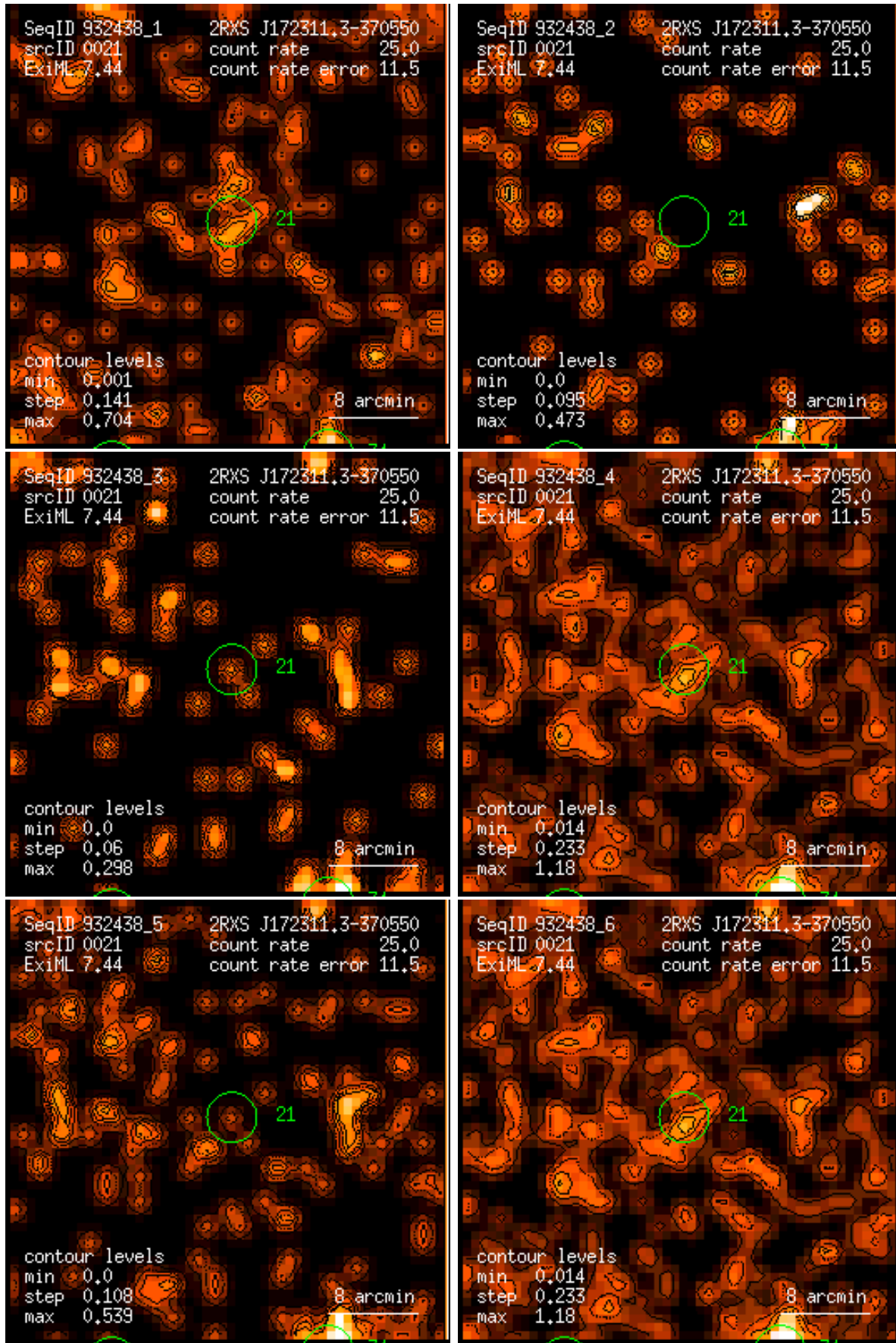
Figure 21: RASS 932438: detection 0021: band rate images, Gaussian filter: (1) PSPC channels 11 – 41, (2) 52 – 90, (3) 91 – 201, (4) 11 – 235, (5) 52 – 201, (6) 11 – 201. Broad band rates in counts/ks. Band rate contour levels in counts/ks/arcmin 2 .
