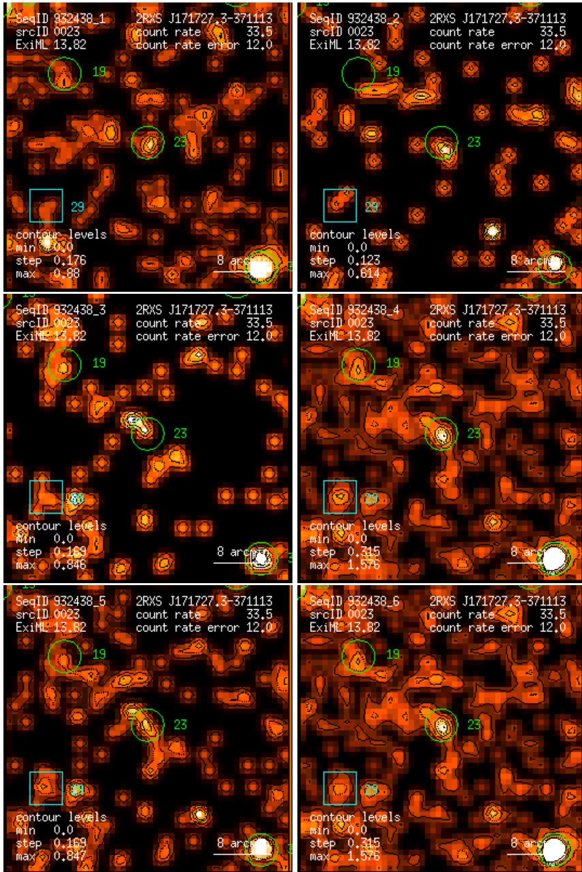
Figure 23: RASS 932438: detection 0023: band rate images, Gaussian filter: (1) PSPC channels 11 – 41, (2) 52 – 90, (3) 91 – 201, (4) 11 – 235, (5) 52 – 201, (6) 11 – 201. Broad band rates in counts/ks. Band rate contour levels in counts/ks/arcmin 2 .
