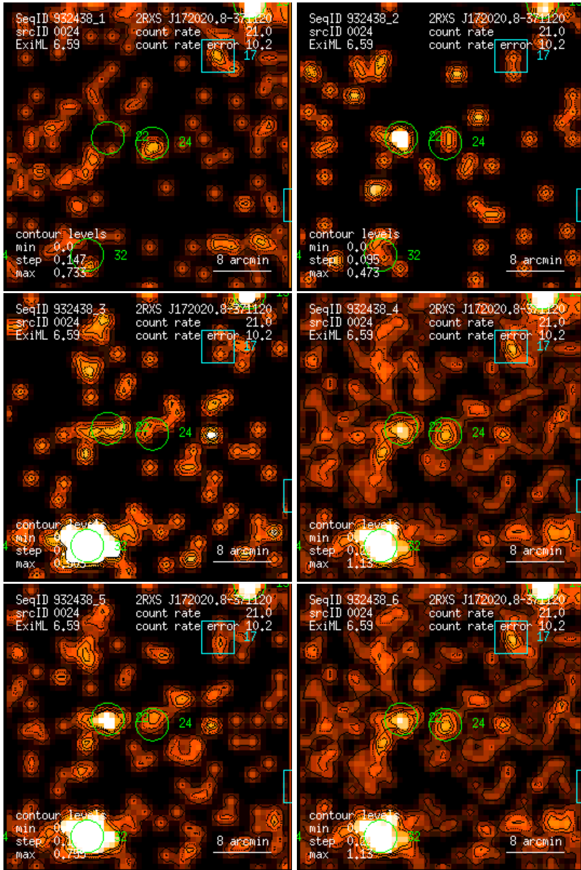
Figure 24: RASS 932438: detection 0024: band rate images, Gaussian filter: (1) PSPC channels 11 – 41, (2) 52 – 90, (3) 91 – 201, (4) 11 – 235, (5) 52 – 201, (6) 11 – 201. Broad band rates in counts/ks. Band rate contour levels in counts/ks/arcmin 2 .
