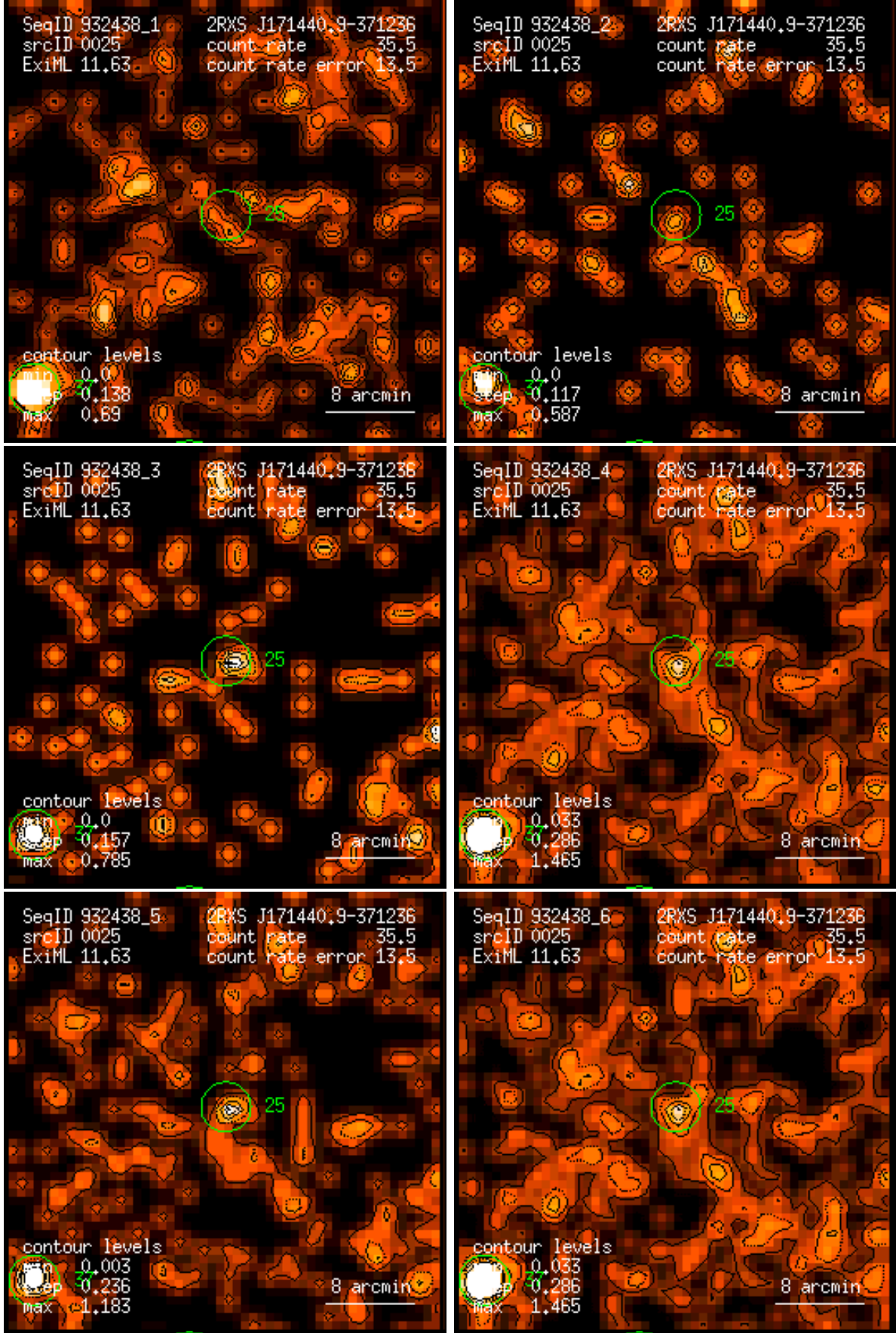
Figure 25: RASS 932438: detection 0025: band rate images, Gaussian filter: (1) PSPC channels 11 – 41, (2) 52 – 90, (3) 91 – 201, (4) 11 – 235, (5) 52 – 201, (6) 11 – 201. Broad band rates in counts/ks. Band rate contour levels in counts/ks/arcmin 2 .
