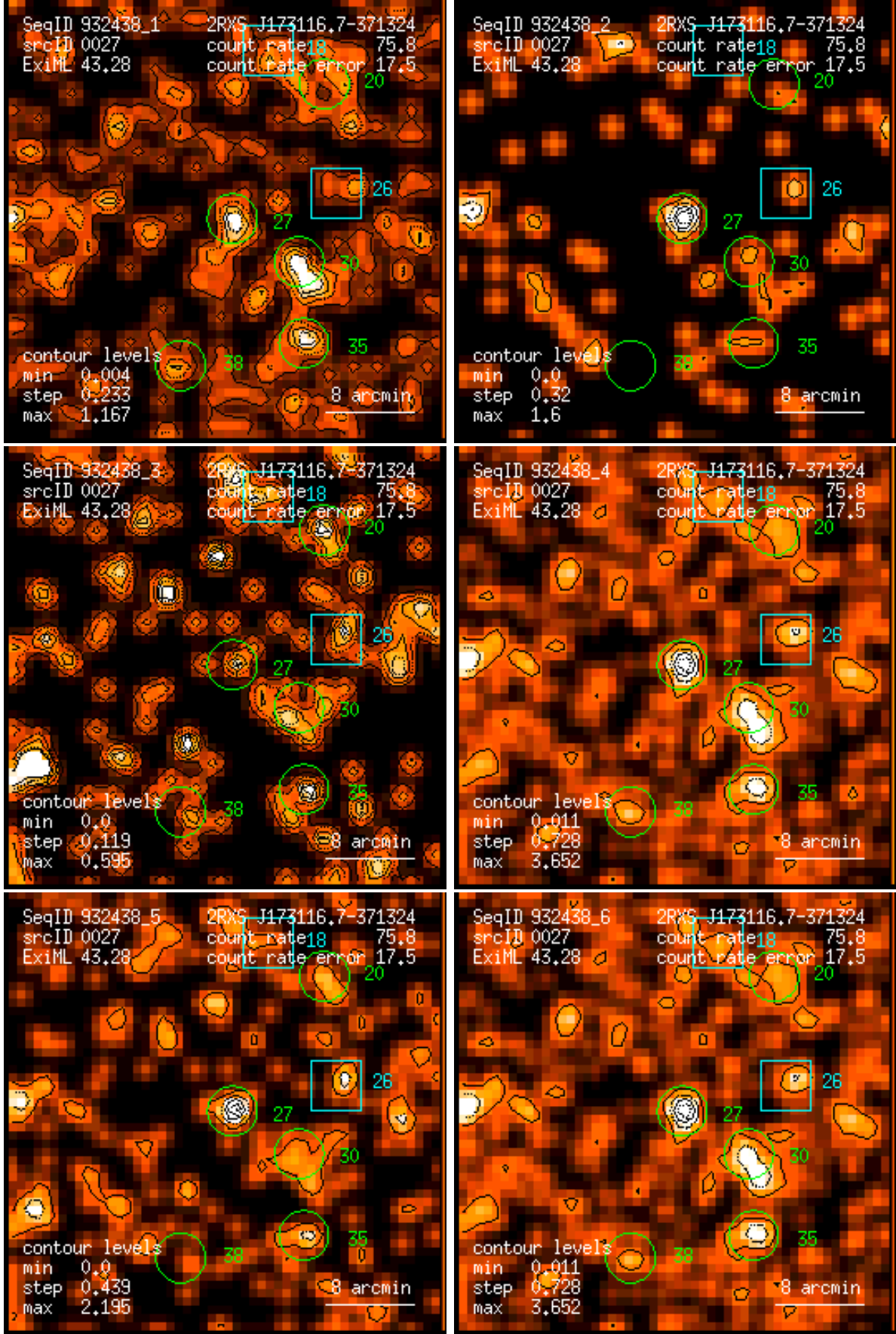
Figure 27: RASS 932438: detection 0027: band rate images, Gaussian filter: (1) PSPC channels 11 – 41, (2) 52 – 90, (3) 91 – 201, (4) 11 – 235, (5) 52 – 201, (6) 11 – 201. Broad band rates in counts/ks. Band rate contour levels in counts/ks/arcmin 2 .
