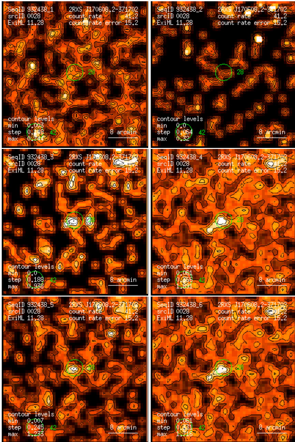
Figure 28: RASS 932438: detection 0028: band rate images, Gaussian filter: (1) PSPC channels 11 – 41, (2) 52 – 90, (3) 91 – 201, (4) 11 – 235, (5) 52 – 201, (6) 11 – 201. Broad band rates in counts/ks. Band rate contour levels in counts/ks/arcmin 2 .
