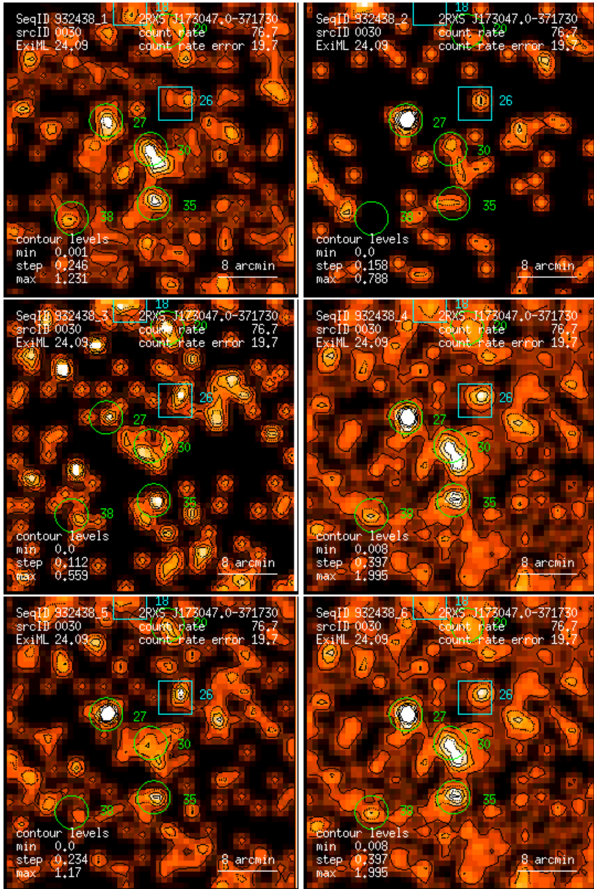
Figure 30: RASS 932438: detection 0030: band rate images, Gaussian filter: (1) PSPC channels 11 – 41, (2) 52 – 90, (3) 91 – 201, (4) 11 – 235, (5) 52 – 201, (6) 11 – 201. Broad band rates in counts/ks. Band rate contour levels in counts/ks/arcmin 2 .
