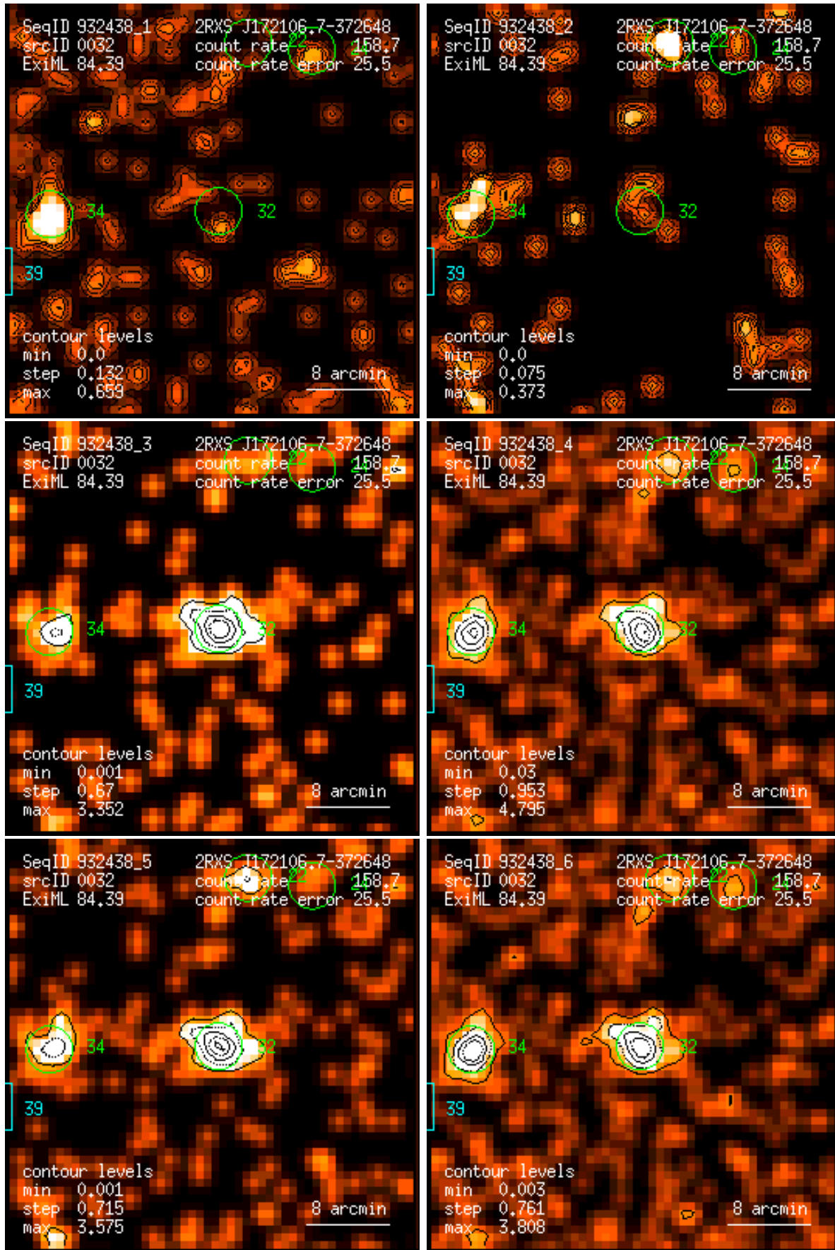
Figure 32: RASS 932438: detection 0032: band rate images, Gaussian filter: (1) PSPC channels 11 – 41, (2) 52 – 90, (3) 91 – 201, (4) 11 – 235, (5) 52 – 201, (6) 11 – 201. Broad band rates in counts/ks. Band rate contour levels in counts/ks/arcmin 2 .
