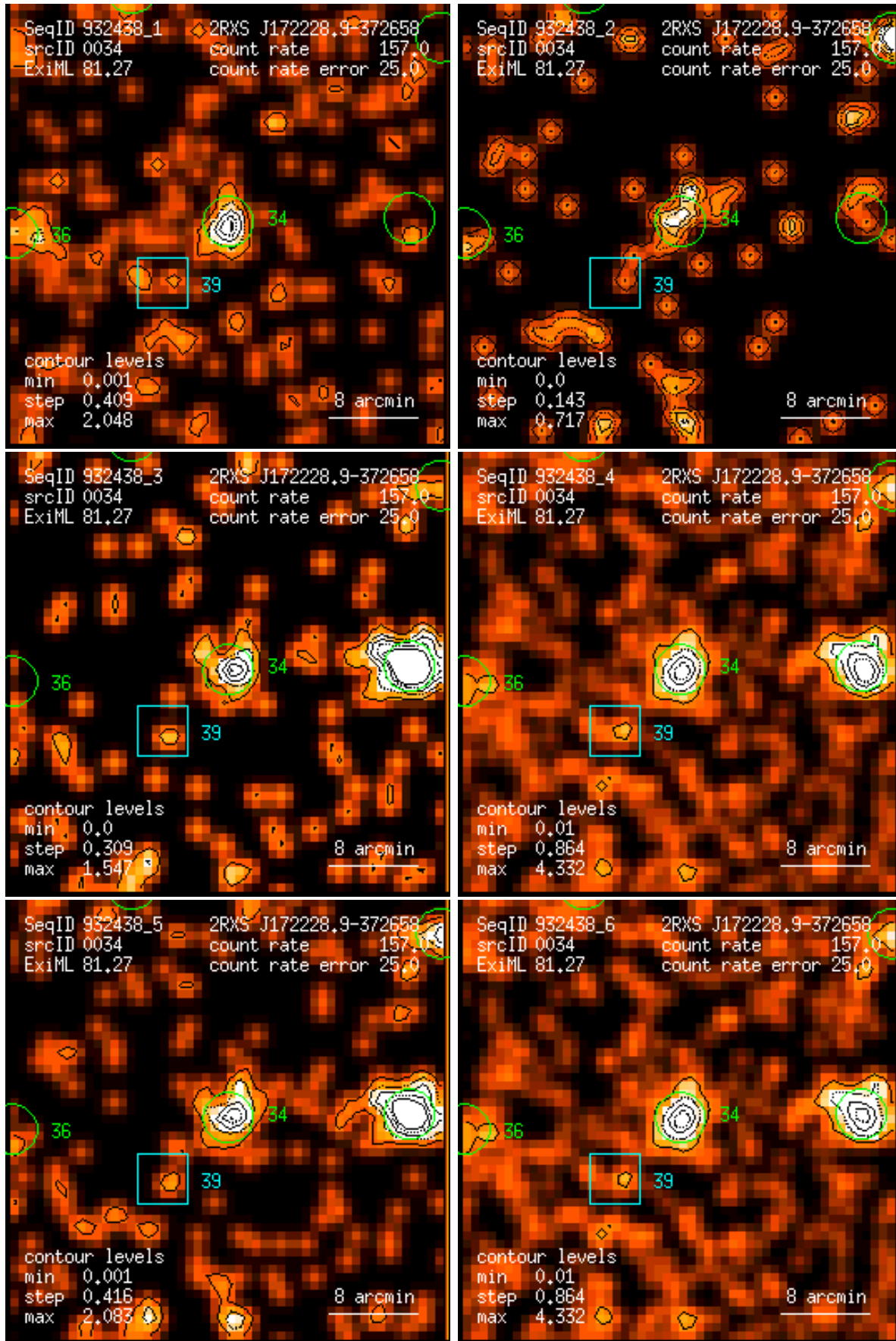
Figure 34: RASS 932438: detection 0034: band rate images, Gaussian filter: (1) PSPC channels 11 – 41, (2) 52 – 90, (3) 91 – 201, (4) 11 – 235, (5) 52 – 201, (6) 11 – 201. Broad band rates in counts/ks. Band rate contour levels in counts/ks/arcmin 2 .
