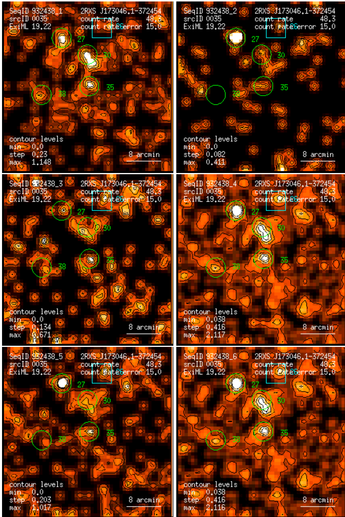
Figure 35: RASS 932438: detection 0035: band rate images, Gaussian filter: (1) PSPC channels 11 – 41, (2) 52 – 90, (3) 91 – 201, (4) 11 – 235, (5) 52 – 201, (6) 11 – 201. Broad band rates in counts/ks. Band rate contour levels in counts/ks/arcmin 2 .
