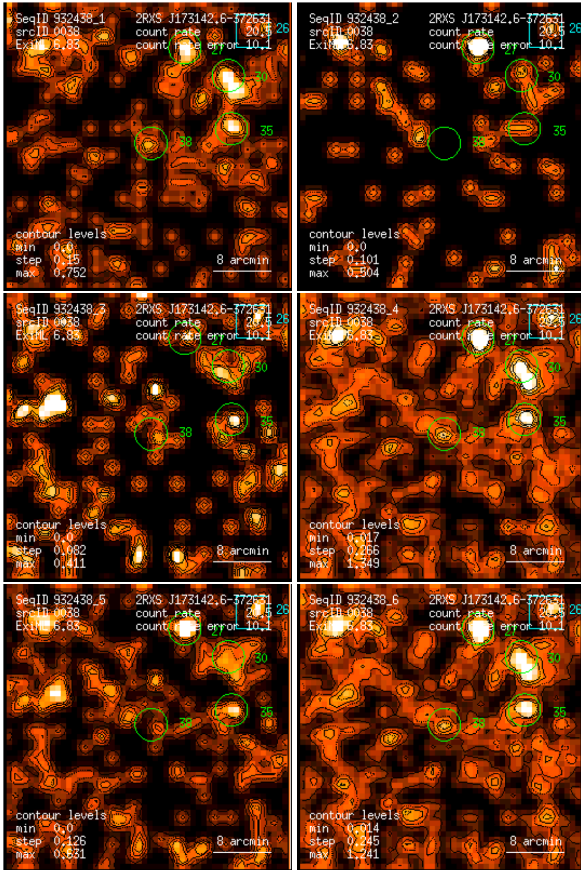
Figure 38: RASS 932438: detection 0038: band rate images, Gaussian filter: (1) PSPC channels 11 – 41, (2) 52 – 90, (3) 91 – 201, (4) 11 – 235, (5) 52 – 201, (6) 11 – 201. Broad band rates in counts/ks. Band rate contour levels in counts/ks/arcmin 2 .
