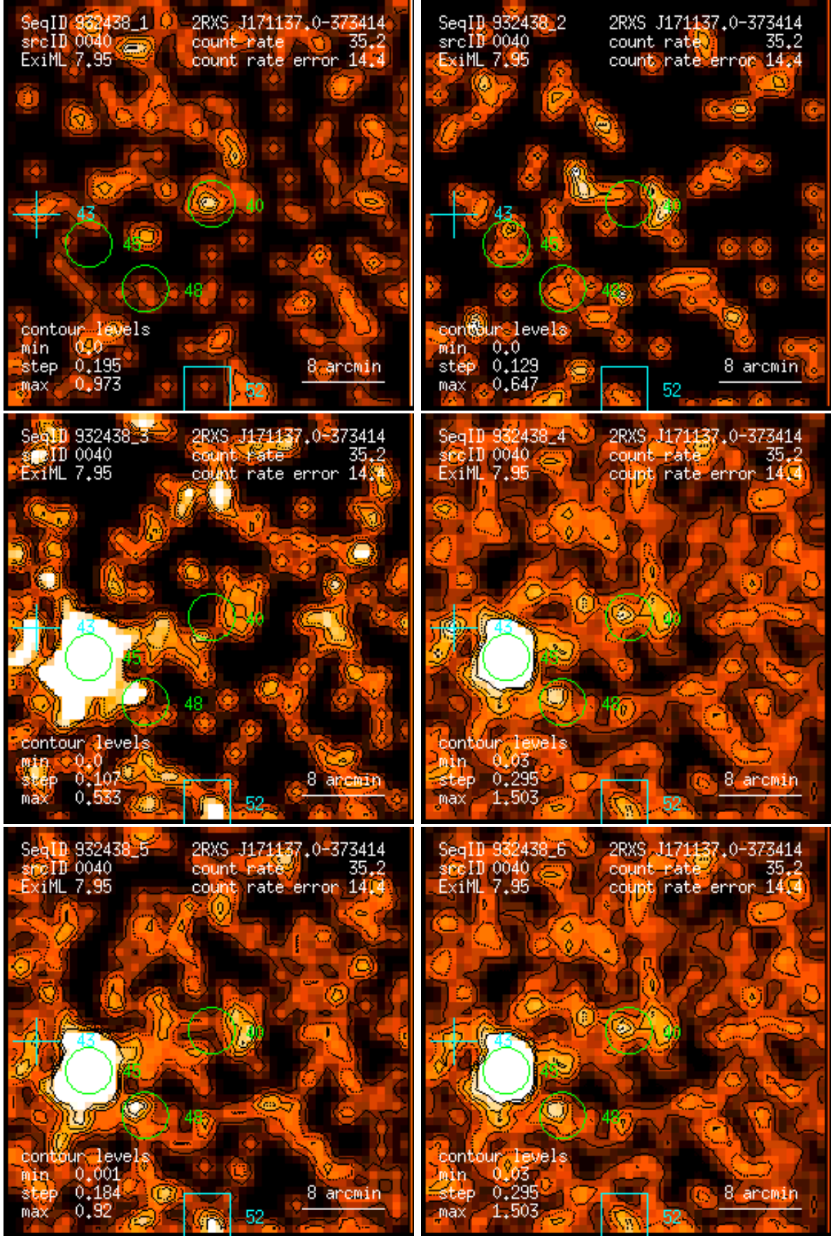
Figure 40: RASS 932438: detection 0040: band rate images, Gaussian filter: (1) PSPC channels 11 – 41, (2) 52 – 90, (3) 91 – 201, (4) 11 – 235, (5) 52 – 201, (6) 11 – 201. Broad band rates in counts/ks. Band rate contour levels in counts/ks/arcmin 2 .
