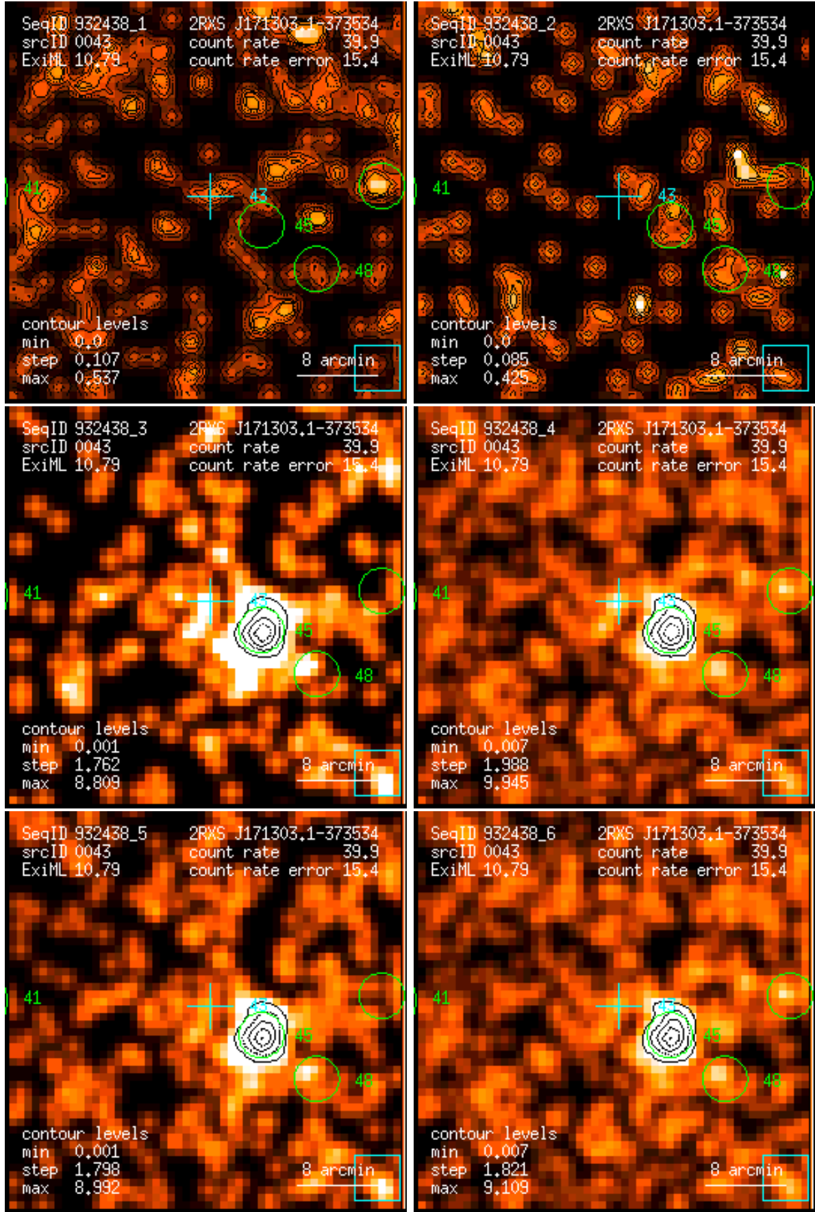
Figure 43: RASS 932438: detection 0043: band rate images, Gaussian filter: (1) PSPC channels 11 – 41, (2) 52 – 90, (3) 91 – 201, (4) 11 – 235, (5) 52 – 201, (6) 11 – 201. Broad band rates in counts/ks. Band rate contour levels in counts/ks/arcmin 2 .
