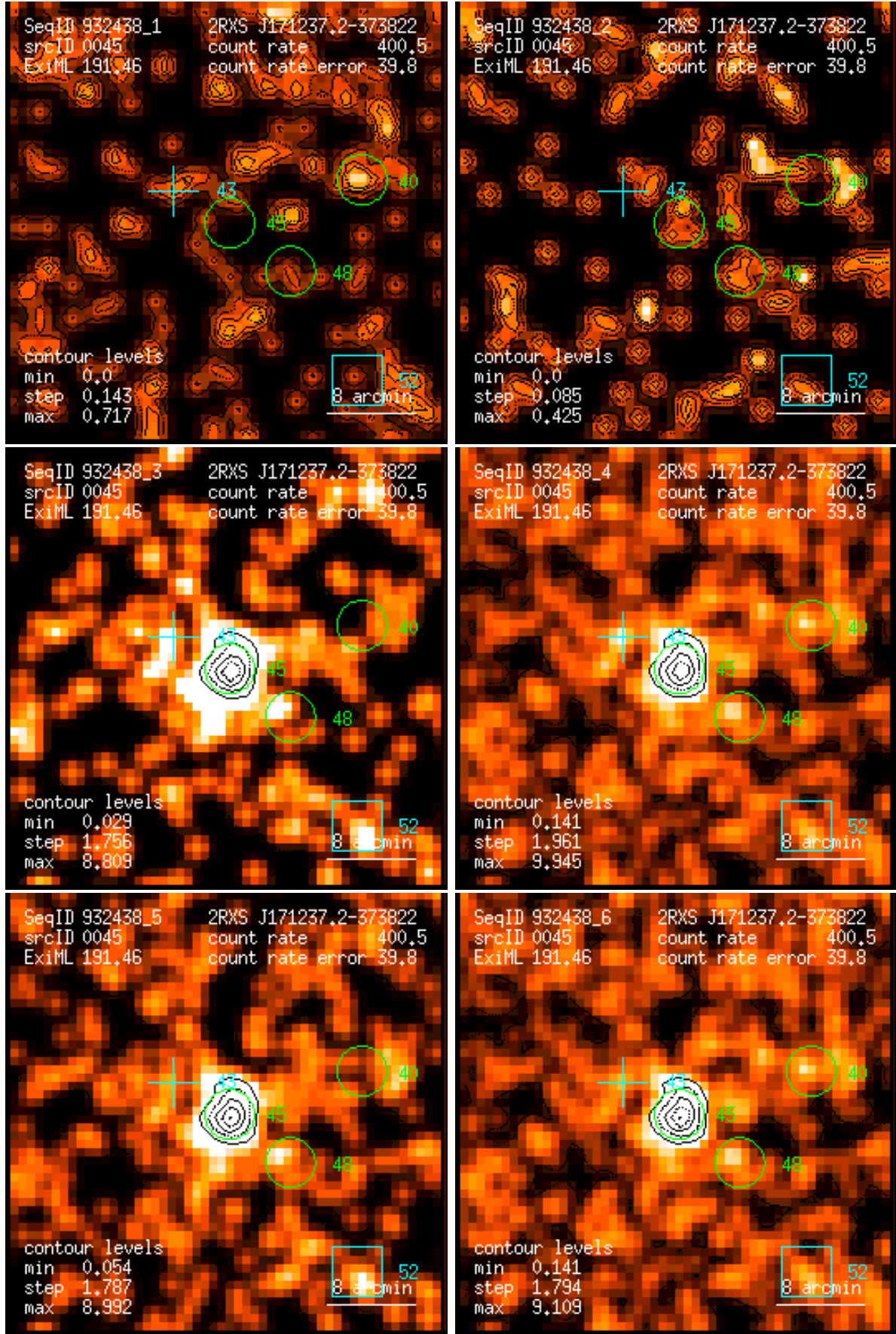
Figure 45: RASS 932438: detection 0045: band rate images, Gaussian filter: (1) PSPC channels 11 – 41, (2) 52 – 90, (3) 91 – 201, (4) 11 – 235, (5) 52 – 201, (6) 11 – 201. Broad band rates in counts/ks. Band rate contour levels in counts/ks/arcmin 2 .
