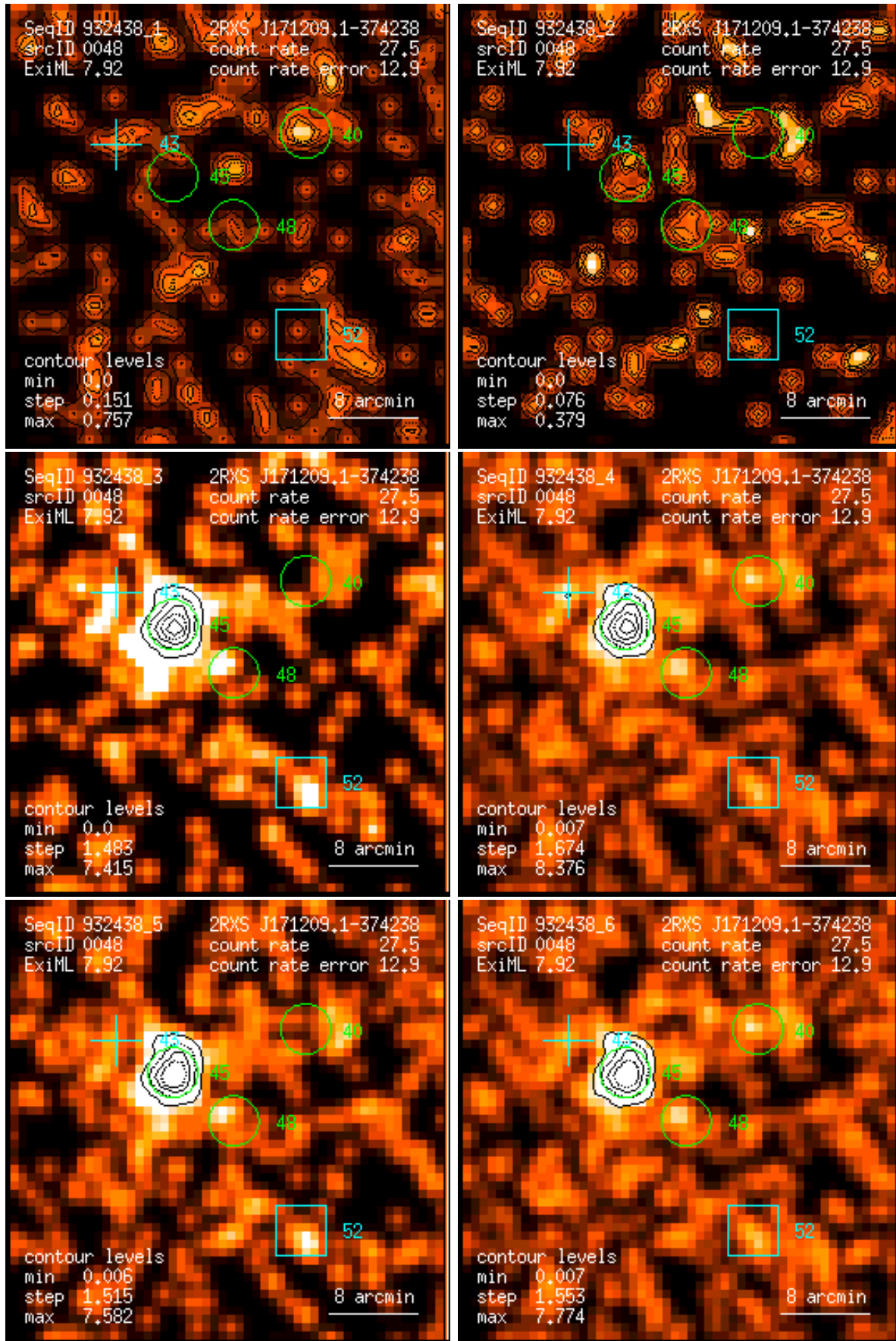
Figure 48: RASS 932438: detection 0048: band rate images, Gaussian filter: (1) PSPC channels 11 – 41, (2) 52 – 90, (3) 91 – 201, (4) 11 – 235, (5) 52 – 201, (6) 11 – 201. Broad band rates in counts/ks. Band rate contour levels in counts/ks/arcmin 2 .
