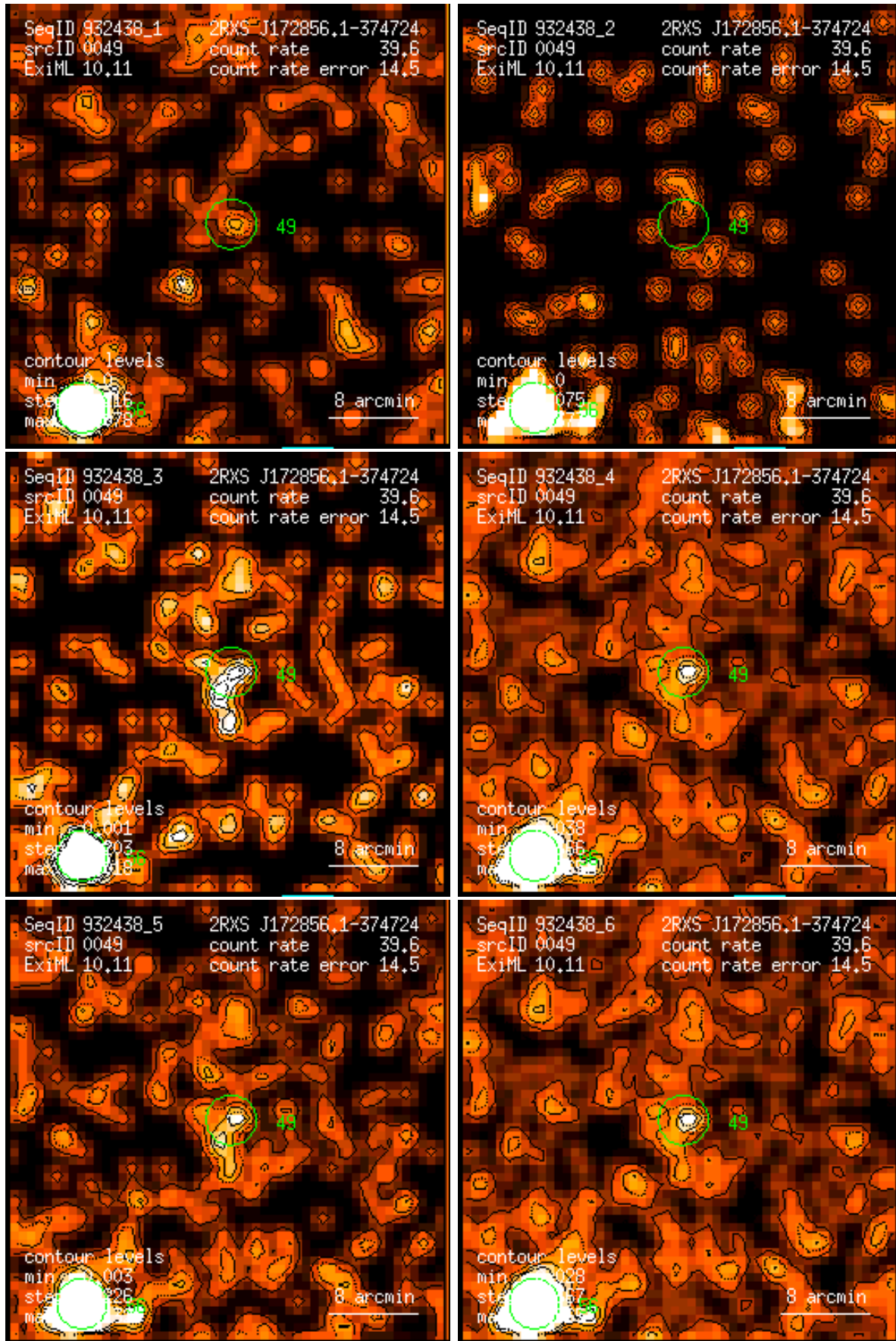
Figure 49: RASS 932438: detection 0049: band rate images, Gaussian filter: (1) PSPC channels 11 – 41, (2) 52 – 90, (3) 91 – 201, (4) 11 – 235, (5) 52 – 201, (6) 11 – 201. Broad band rates in counts/ks. Band rate contour levels in counts/ks/arcmin 2 .
