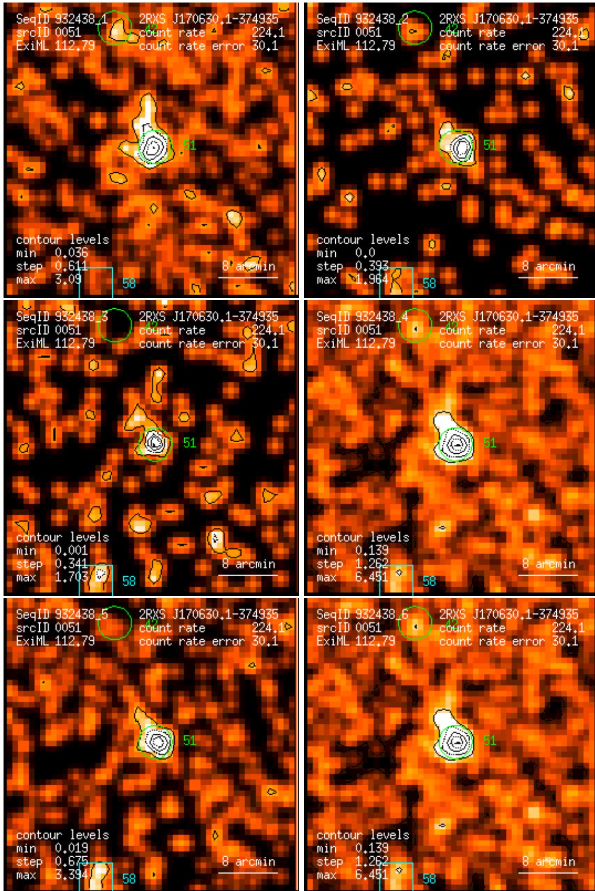
Figure 51: RASS 932438: detection 0051: band rate images, Gaussian filter: (1) PSPC channels 11 – 41, (2) 52 – 90, (3) 91 – 201, (4) 11 – 235, (5) 52 – 201, (6) 11 – 201. Broad band rates in counts/ks. Band rate contour levels in counts/ks/arcmin 2 .
