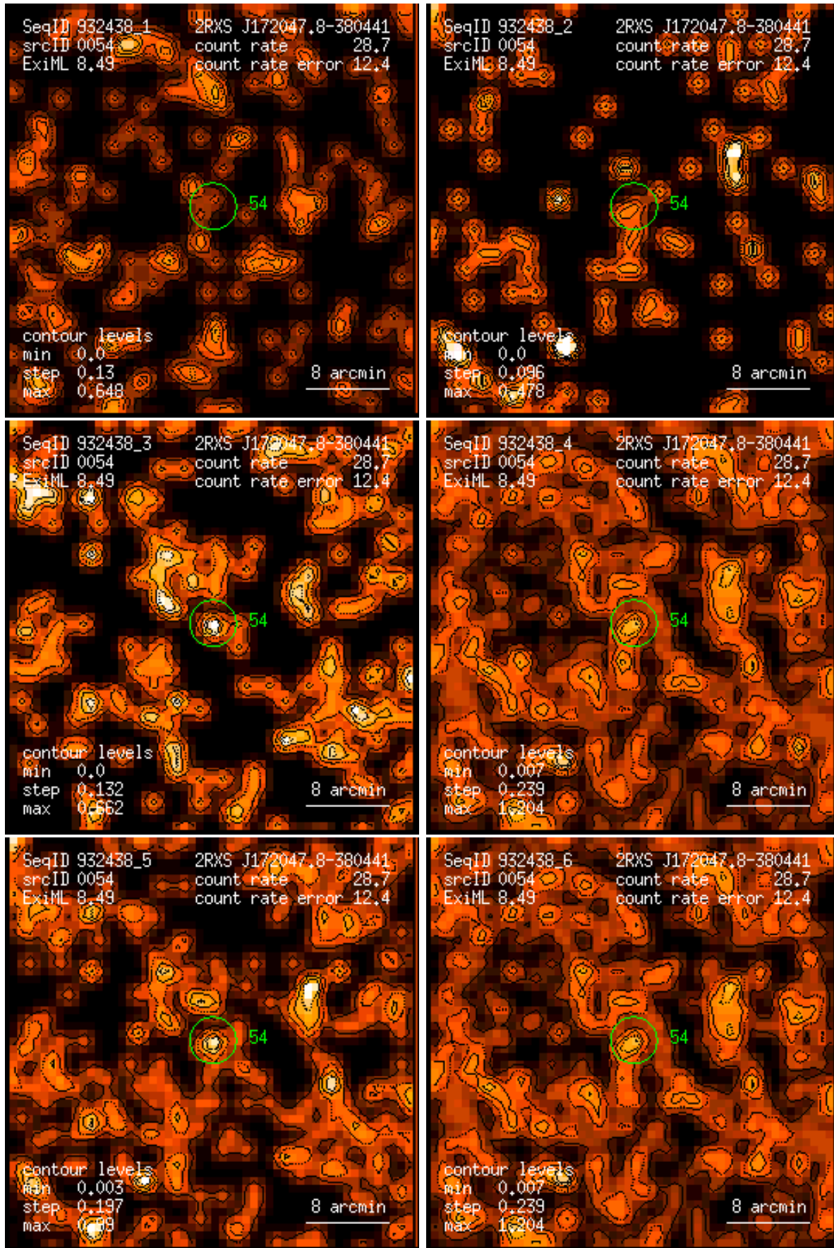
Figure 54: RASS 932438: detection 0054: band rate images, Gaussian filter: (1) PSPC channels 11 – 41, (2) 52 – 90, (3) 91 – 201, (4) 11 – 235, (5) 52 – 201, (6) 11 – 201. Broad band rates in counts/ks. Band rate contour levels in counts/ks/arcmin 2 .
