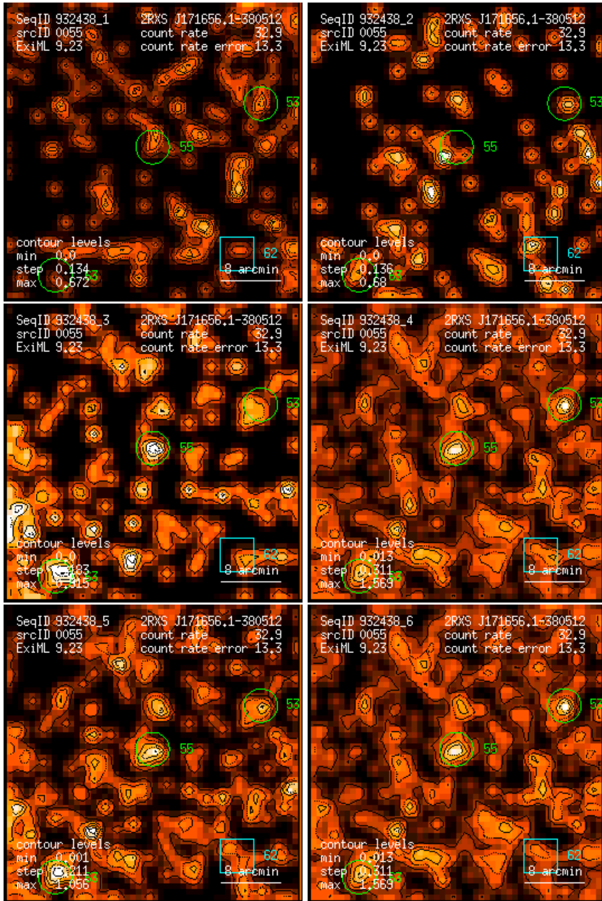
Figure 55: RASS 932438: detection 0055: band rate images, Gaussian filter: (1) PSPC channels 11 – 41, (2) 52 – 90, (3) 91 – 201, (4) 11 – 235, (5) 52 – 201, (6) 11 – 201. Broad band rates in counts/ks. Band rate contour levels in counts/ks/arcmin 2 .
