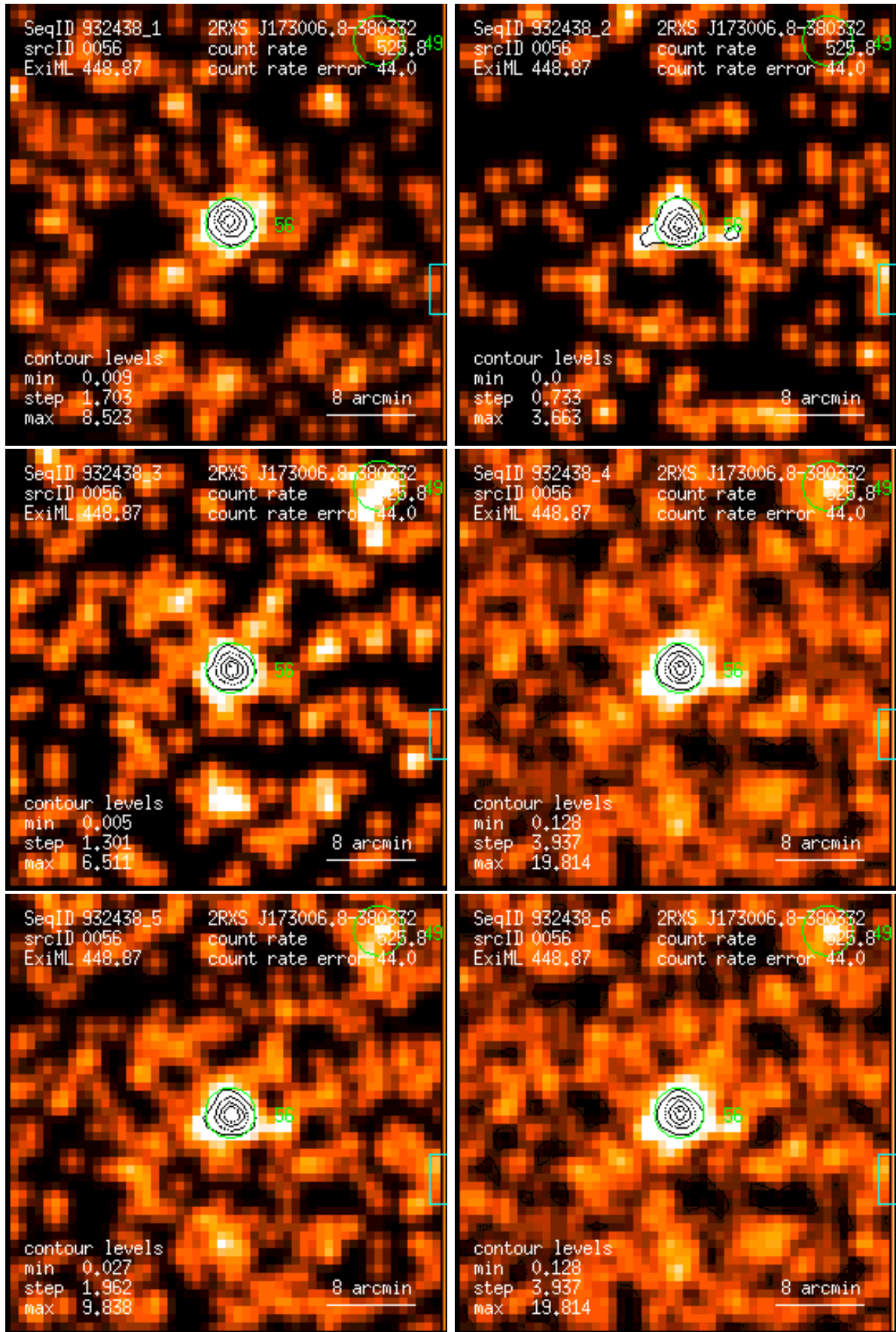
Figure 56: RASS 932438: detection 0056: band rate images, Gaussian filter: (1) PSPC channels 11 – 41, (2) 52 – 90, (3) 91 – 201, (4) 11 – 235, (5) 52 – 201, (6) 11 – 201. Broad band rates in counts/ks. Band rate contour levels in counts/ks/arcmin 2 .
