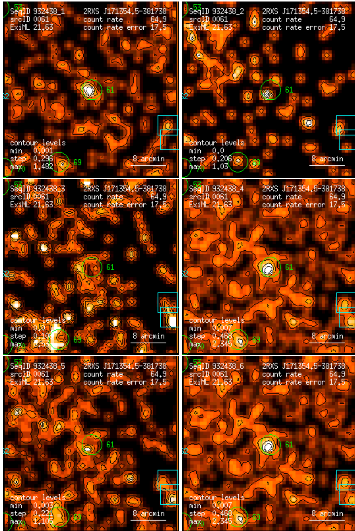
Figure 61: RASS 932438: detection 0061: band rate images, Gaussian filter: (1) PSPC channels 11 – 41, (2) 52 – 90, (3) 91 – 201, (4) 11 – 235, (5) 52 – 201, (6) 11 – 201. Broad band rates in counts/ks. Band rate contour levels in counts/ks/arcmin 2 .
