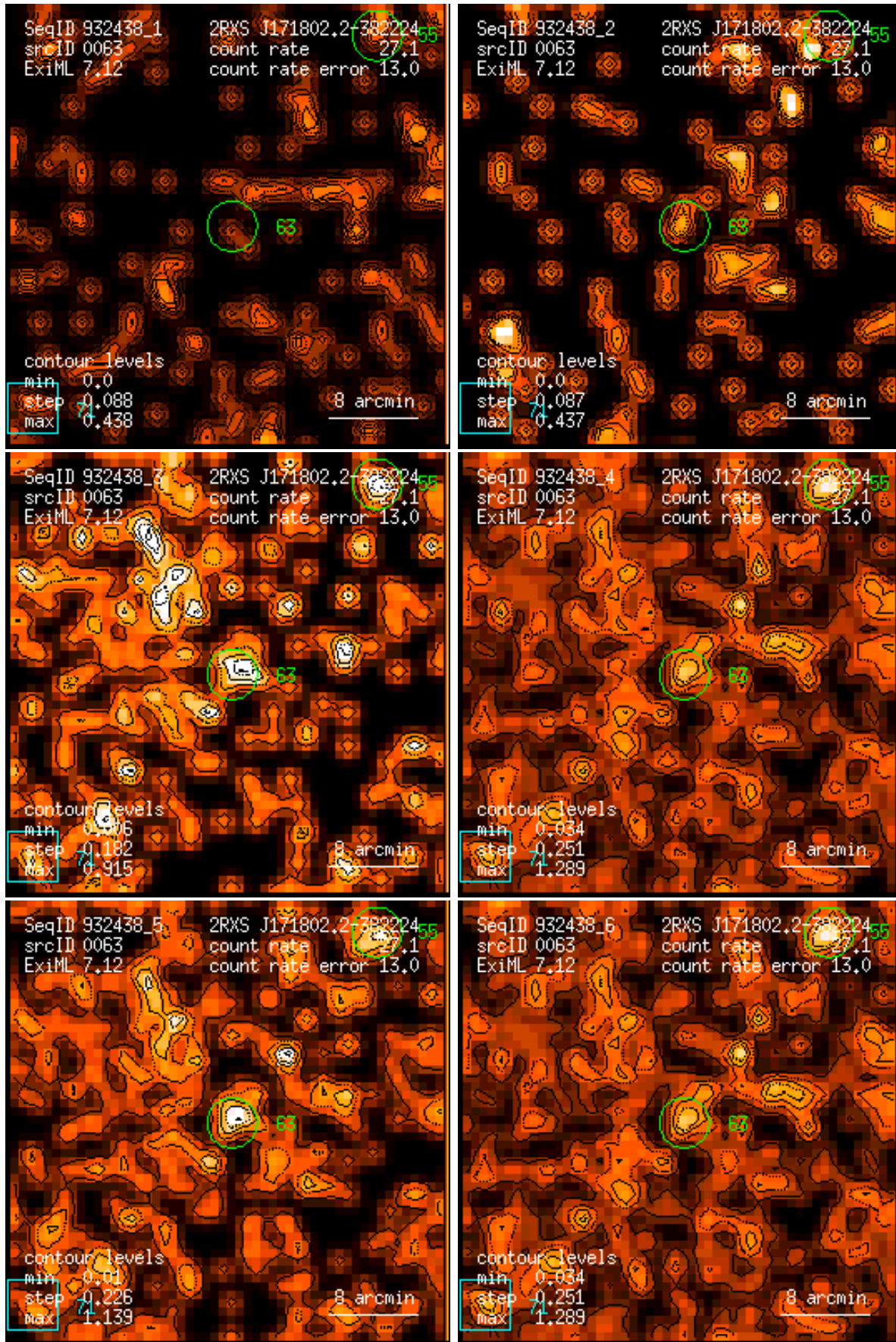
Figure 63: RASS 932438: detection 0063: band rate images, Gaussian filter: (1) PSPC channels 11 – 41, (2) 52 – 90, (3) 91 – 201, (4) 11 – 235, (5) 52 – 201, (6) 11 – 201. Broad band rates in counts/ks. Band rate contour levels in counts/ks/arcmin 2 .
