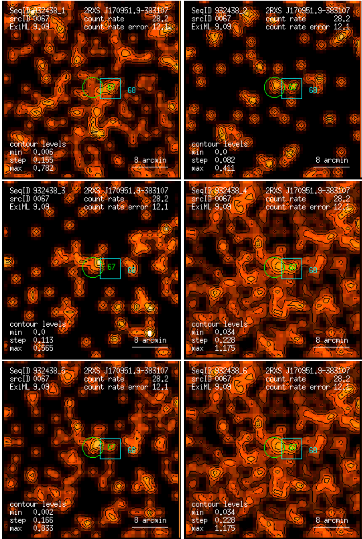
Figure 67: RASS 932438: detection 0067: band rate images, Gaussian filter: (1) PSPC channels 11 – 41, (2) 52 – 90, (3) 91 – 201, (4) 11 – 235, (5) 52 – 201, (6) 11 – 201. Broad band rates in counts/ks. Band rate contour levels in counts/ks/arcmin 2 .
