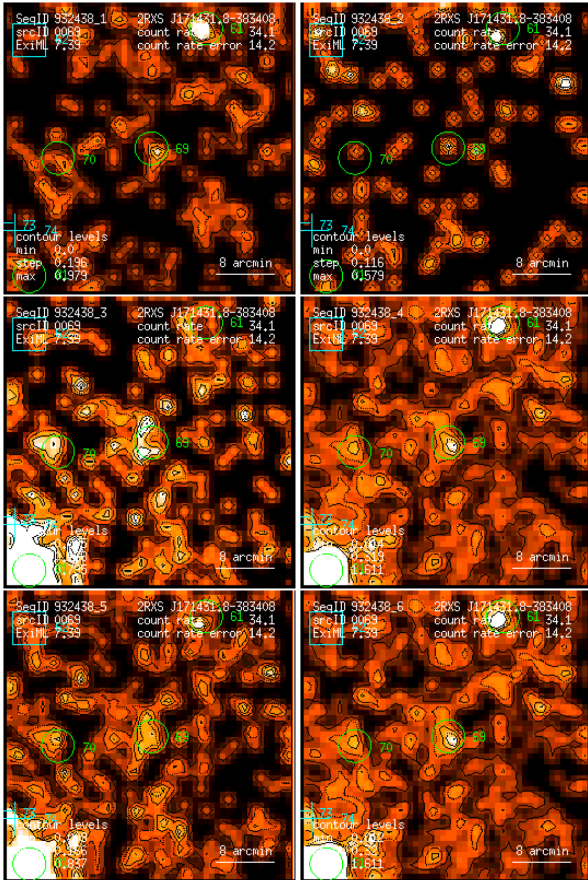
Figure 69: RASS 932438: detection 0069: band rate images, Gaussian filter: (1) PSPC channels 11 – 41, (2) 52 – 90, (3) 91 – 201, (4) 11 – 235, (5) 52 – 201, (6) 11 – 201. Broad band rates in counts/ks. Band rate contour levels in counts/ks/arcmin 2 .
