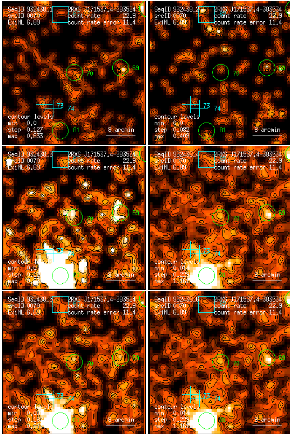
Figure 70: RASS 932438: detection 0070: band rate images, Gaussian filter: (1) PSPC channels 11 – 41, (2) 52 – 90, (3) 91 – 201, (4) 11 – 235, (5) 52 – 201, (6) 11 – 201. Broad band rates in counts/ks. Band rate contour levels in counts/ks/arcmin 2 .
