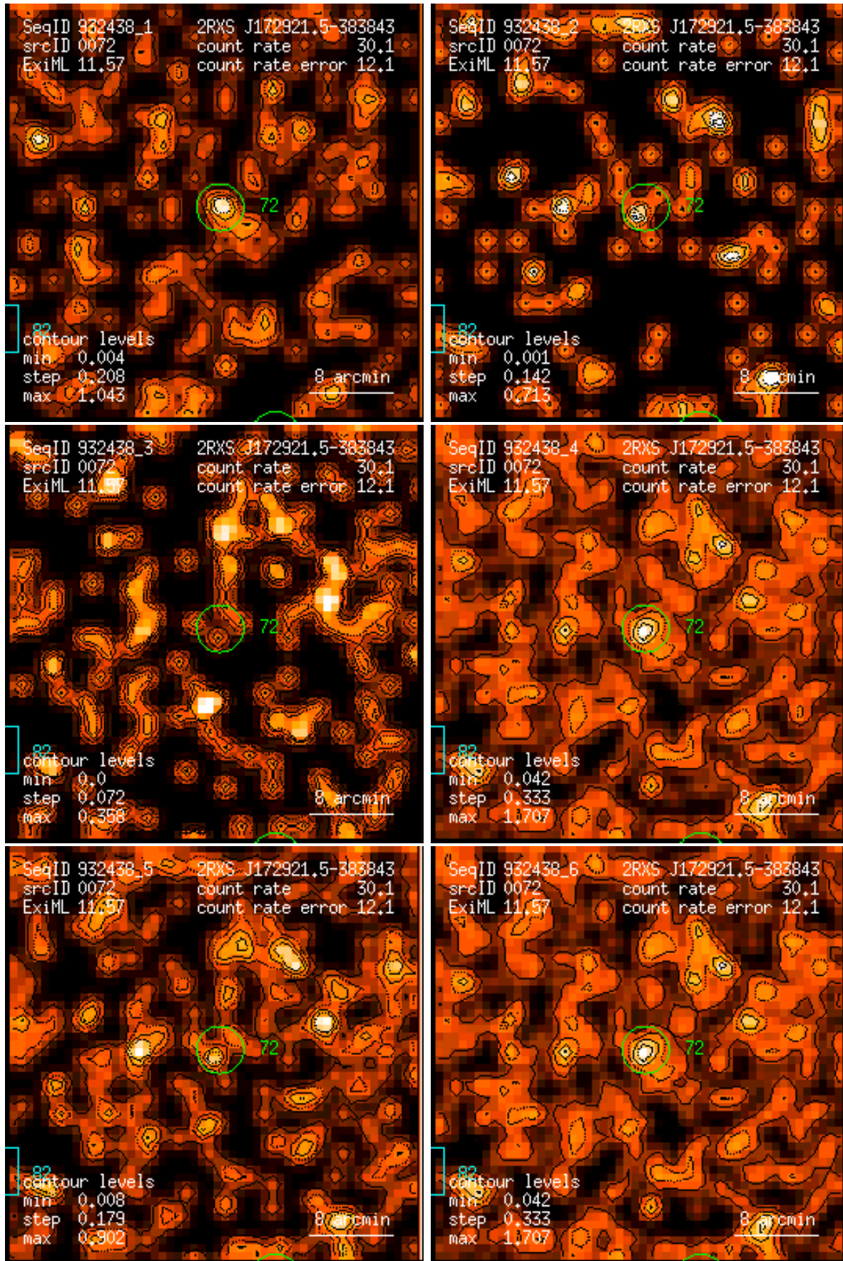
Figure 72: RASS 932438: detection 0072: band rate images, Gaussian filter: (1) PSPC channels 11 – 41, (2) 52 – 90, (3) 91 – 201, (4) 11 – 235, (5) 52 – 201, (6) 11 – 201. Broad band rates in counts/ks. Band rate contour levels in counts/ks/arcmin 2 .
