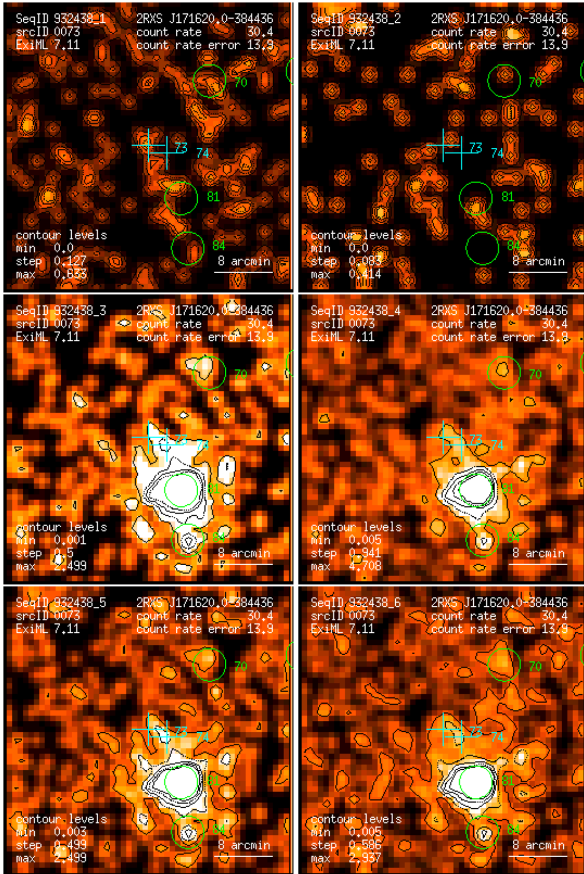
Figure 73: RASS 932438: detection 0073: band rate images, Gaussian filter: (1) PSPC channels 11 – 41, (2) 52 – 90, (3) 91 – 201, (4) 11 – 235, (5) 52 – 201, (6) 11 – 201. Broad band rates in counts/ks. Band rate contour levels in counts/ks/arcmin 2 .
