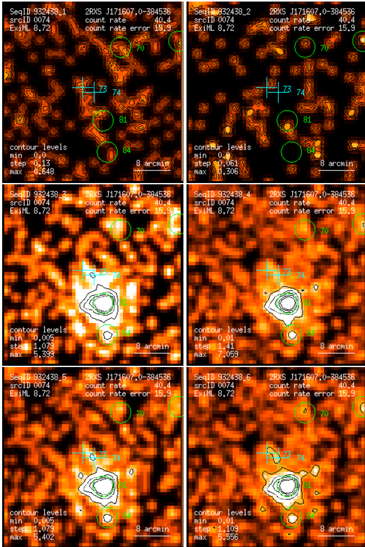
Figure 74: RASS 932438: detection 0074: band rate images, Gaussian filter: (1) PSPC channels 11 – 41, (2) 52 – 90, (3) 91 – 201, (4) 11 – 235, (5) 52 – 201, (6) 11 – 201. Broad band rates in counts/ks. Band rate contour levels in counts/ks/arcmin 2 .
