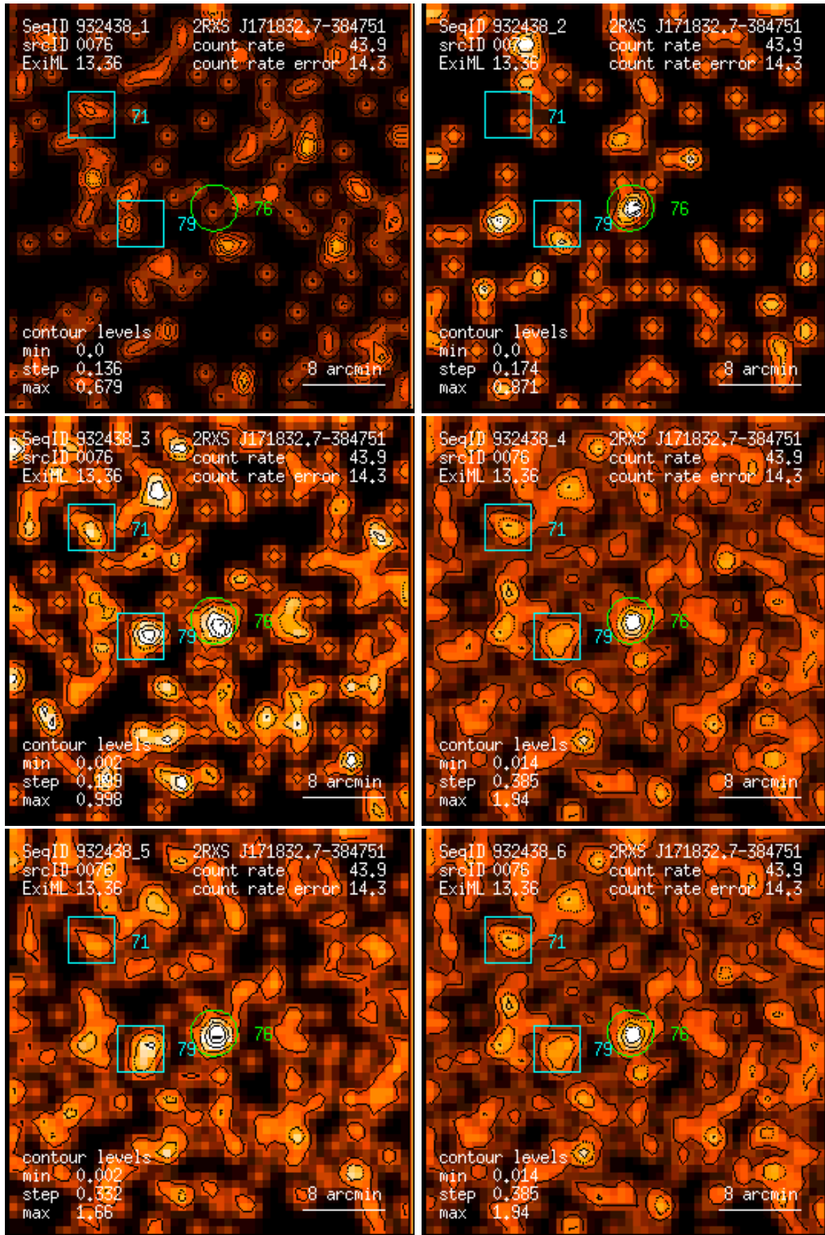
Figure 76: RASS 932438: detection 0076: band rate images, Gaussian filter: (1) PSPC channels 11 – 41, (2) 52 – 90, (3) 91 – 201, (4) 11 – 235, (5) 52 – 201, (6) 11 – 201. Broad band rates in counts/ks. Band rate contour levels in counts/ks/arcmin 2 .
