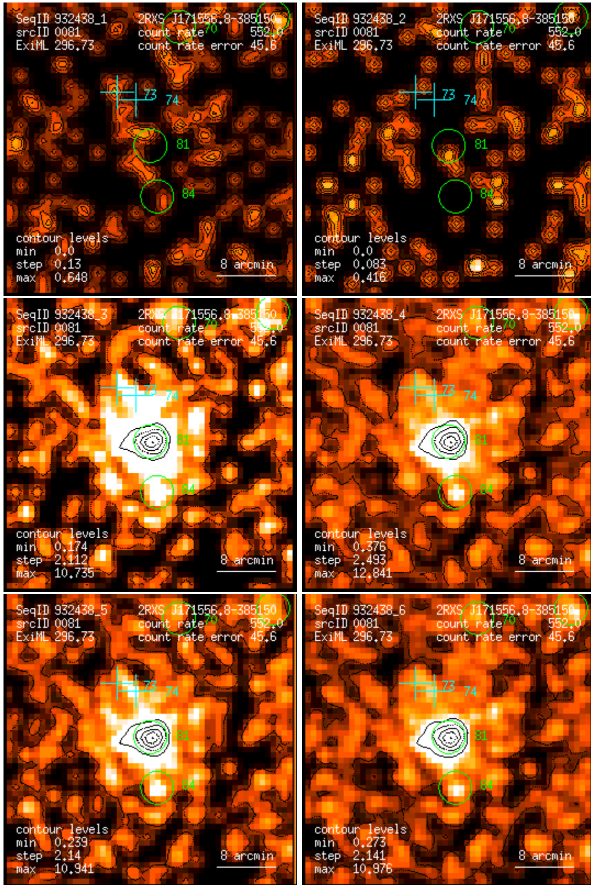
Figure 81: RASS 932438: detection 0081: band rate images, Gaussian filter: (1) PSPC channels 11 – 41, (2) 52 – 90, (3) 91 – 201, (4) 11 – 235, (5) 52 – 201, (6) 11 – 201. Broad band rates in counts/ks. Band rate contour levels in counts/ks/arcmin 2 .
