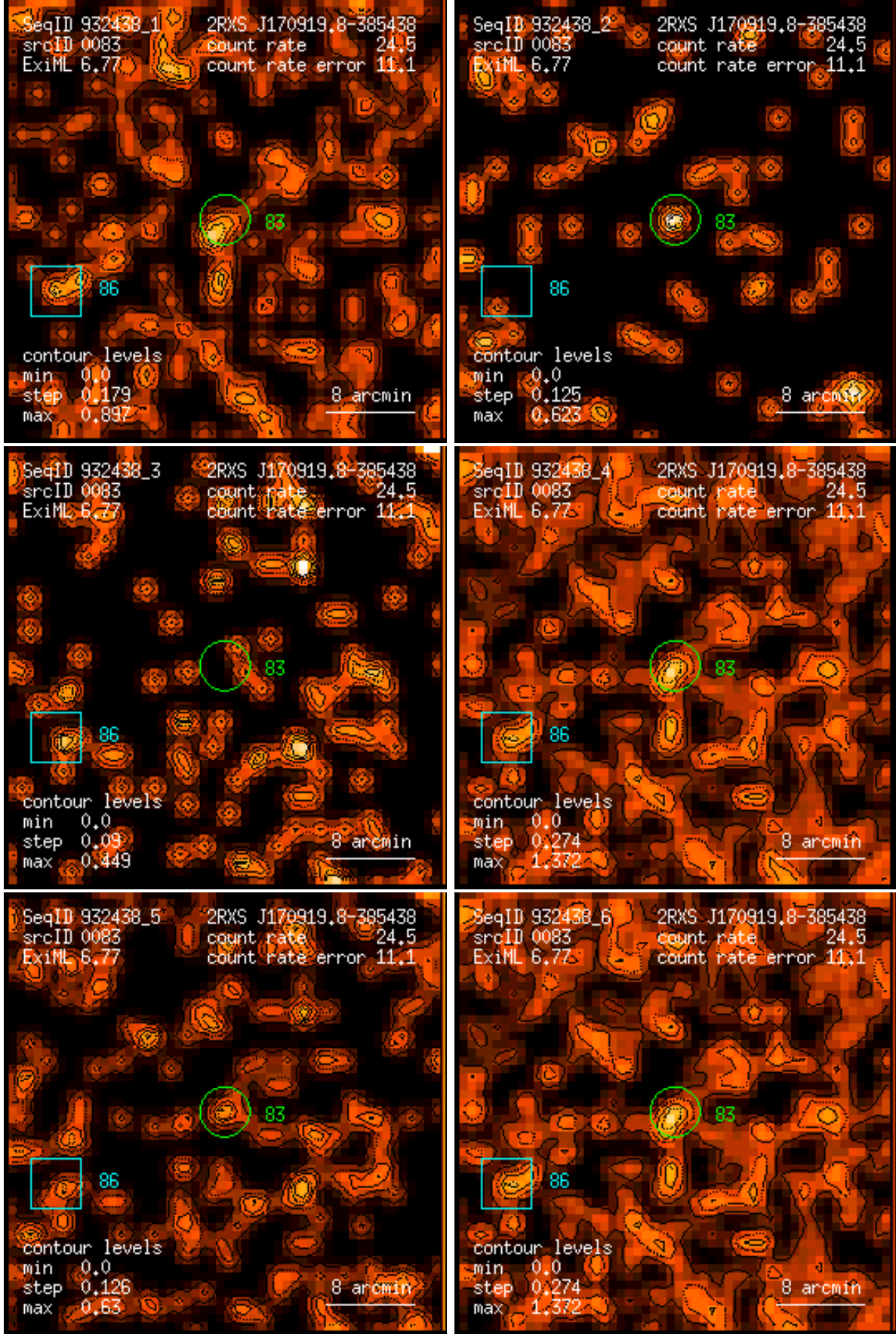
Figure 83: RASS 932438: detection 0083: band rate images, Gaussian filter: (1) PSPC channels 11 – 41, (2) 52 – 90, (3) 91 – 201, (4) 11 – 235, (5) 52 – 201, (6) 11 – 201. Broad band rates in counts/ks. Band rate contour levels in counts/ks/arcmin 2 .
