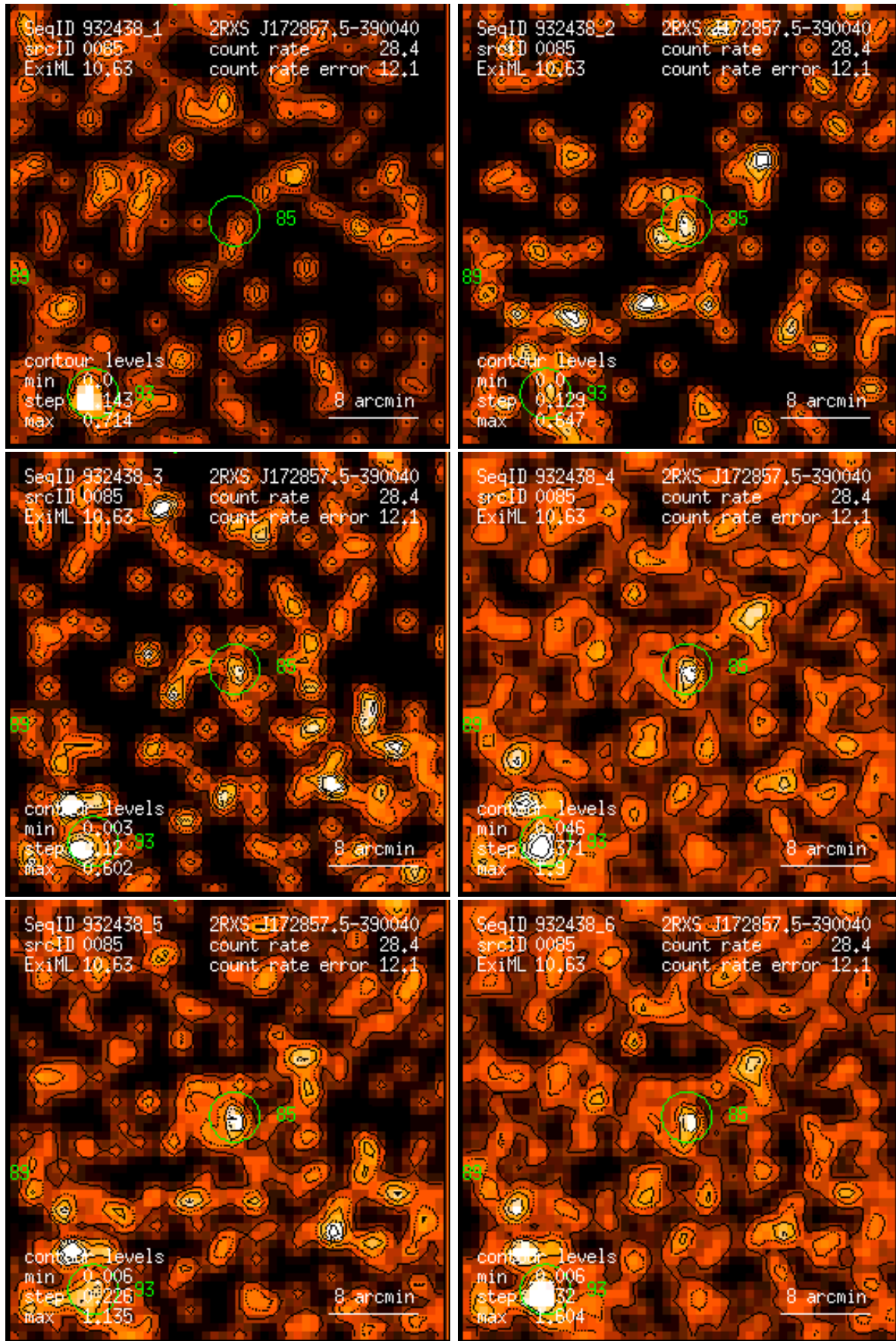
Figure 85: RASS 932438: detection 0085: band rate images, Gaussian filter: (1) PSPC channels 11 – 41, (2) 52 – 90, (3) 91 – 201, (4) 11 – 235, (5) 52 – 201, (6) 11 – 201. Broad band rates in counts/ks. Band rate contour levels in counts/ks/arcmin 2 .
