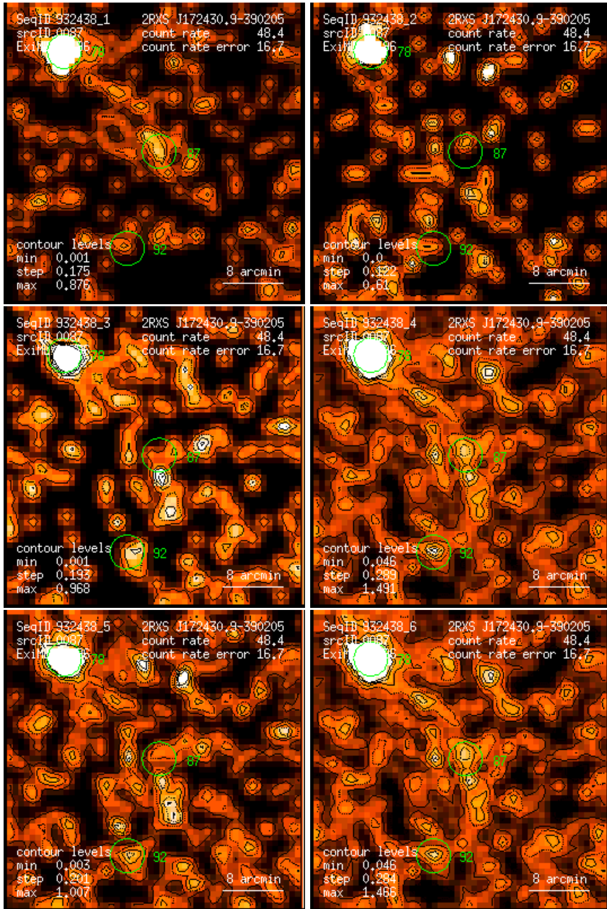
Figure 87: RASS 932438: detection 0087: band rate images, Gaussian filter: (1) PSPC channels 11 – 41, (2) 52 – 90, (3) 91 – 201, (4) 11 – 235, (5) 52 – 201, (6) 11 – 201. Broad band rates in counts/ks. Band rate contour levels in counts/ks/arcmin 2 .
