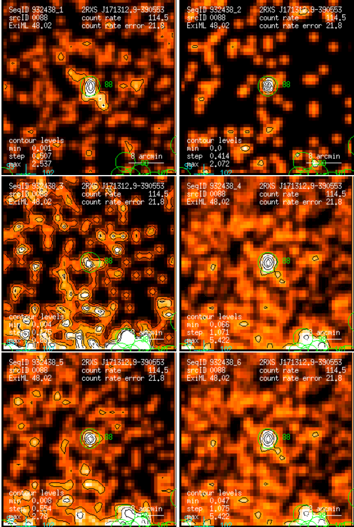
Figure 88: RASS 932438: detection 0088: band rate images, Gaussian filter: (1) PSPC channels 11 – 41, (2) 52 – 90, (3) 91 – 201, (4) 11 – 235, (5) 52 – 201, (6) 11 – 201. Broad band rates in counts/ks. Band rate contour levels in counts/ks/arcmin 2 .
