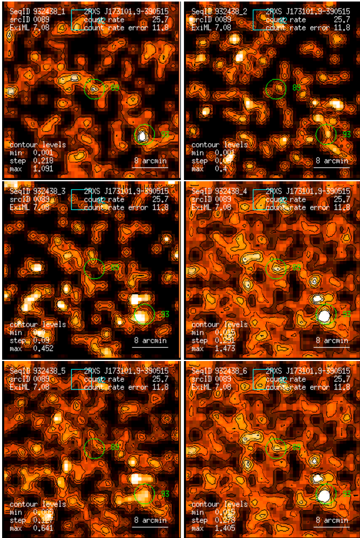
Figure 89: RASS 932438: detection 0089: band rate images, Gaussian filter: (1) PSPC channels 11 – 41, (2) 52 – 90, (3) 91 – 201, (4) 11 – 235, (5) 52 – 201, (6) 11 – 201. Broad band rates in counts/ks. Band rate contour levels in counts/ks/arcmin 2 .
