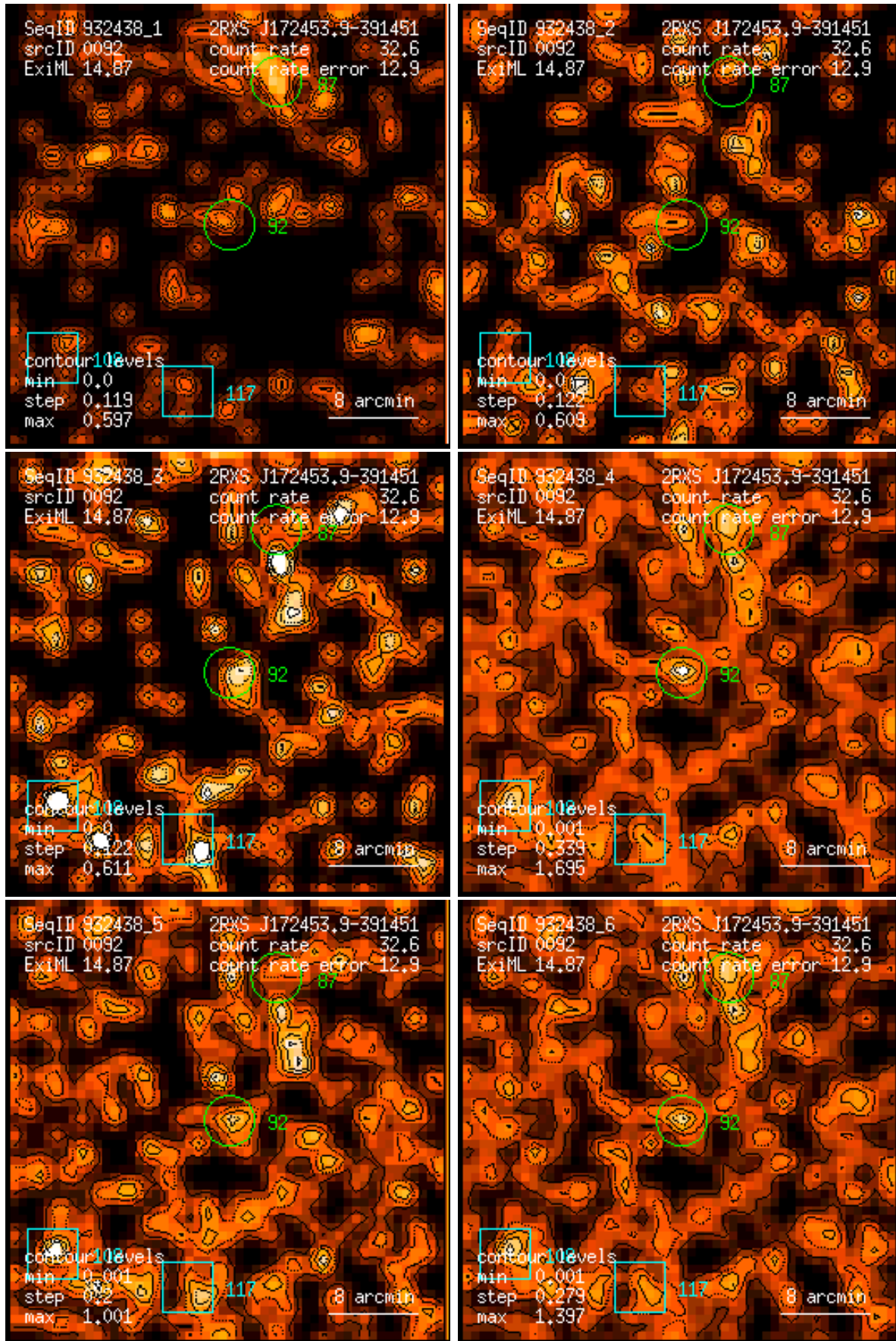
Figure 92: RASS 932438: detection 0092: band rate images, Gaussian filter: (1) PSPC channels 11 – 41, (2) 52 – 90, (3) 91 – 201, (4) 11 – 235, (5) 52 – 201, (6) 11 – 201. Broad band rates in counts/ks. Band rate contour levels in counts/ks/arcmin 2 .
