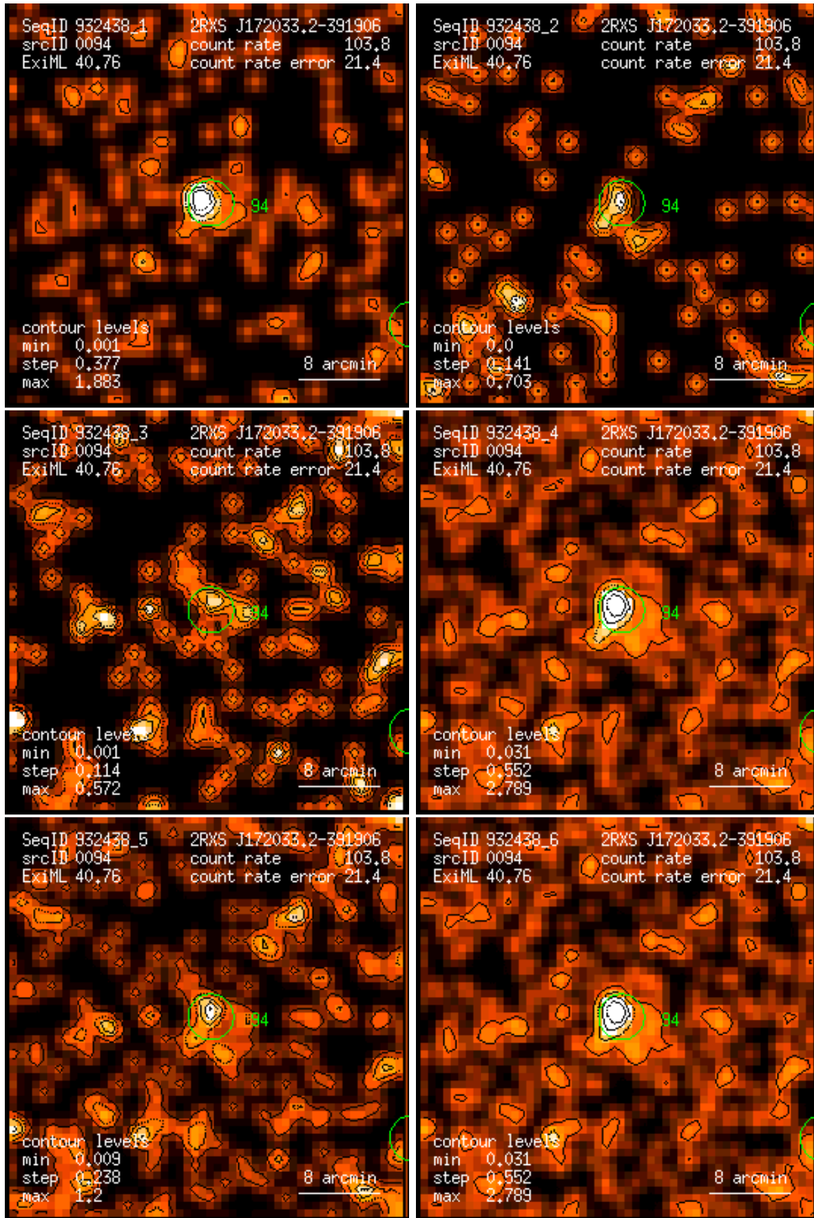
Figure 94: RASS 932438: detection 0094: band rate images, Gaussian filter: (1) PSPC channels 11 – 41, (2) 52 – 90, (3) 91 – 201, (4) 11 – 235, (5) 52 – 201, (6) 11 – 201. Broad band rates in counts/ks. Band rate contour levels in counts/ks/arcmin 2 .
